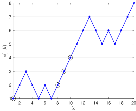
Fig. 1. Partial balance s(1, k) versus k for n = 10 and \mathbf{x} = (1, 1, 1, -1, -1, 1, -1, 1, 1, 1) . The diagram shows s(1, k) in the extended interval 1 \leq k \leq 2n , by letting x_{n+p} = x_p for 1 \leq p \leq n , which makes it more convenient to peruse the partial balances s(i, k) for any i , as explained in the text. The minimal indexes of \mathbf{x} are the k -values of the points indicated by the circles.
