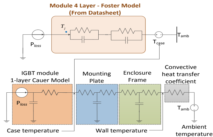
Figure 14. Lumped element thermal network model for the system shown in Figure 2 [11].
