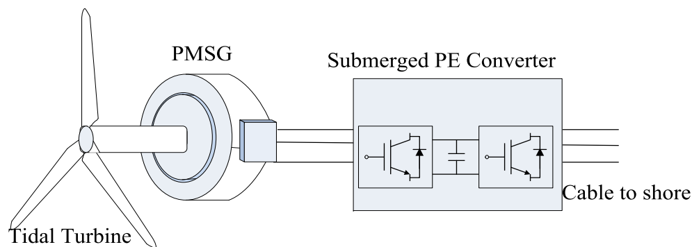
Figure 1. Tidal turbine drive train with a direct-drive permanent magnet synchronous generator (PMSG) and a power electronic (PE) converter.
