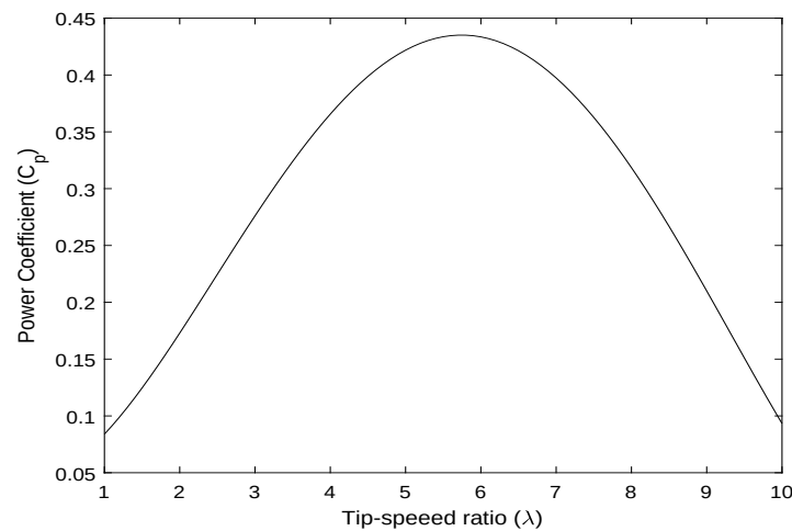
Figure 7. C_p - \lambda curve for the tidal turbine; adapted from Reference [43].
