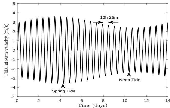
Figure 4. Tidal stream velocity profile at a typical tidal site experiencing semi-diurnal tides.
