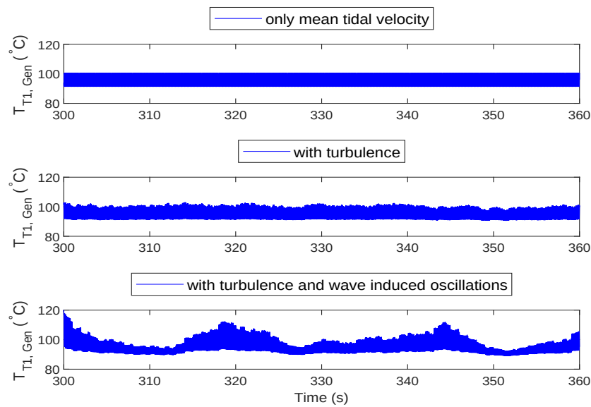
Figure 19. Temperature of the Generator Side Converter insulated gate bipolar transistor (IGBT) (T1) as a function of the fluctuations in the tidal stream velocity.
