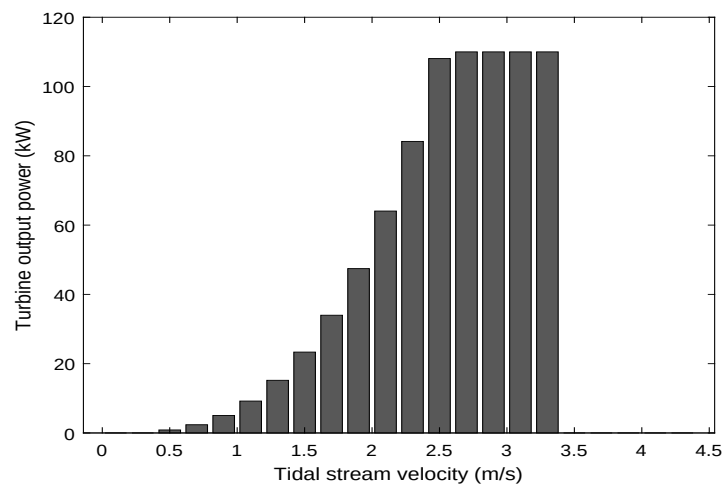
Figure 8. Power curve of the fixed pitch tidal turbine as a function of the tidal stream velocity.
