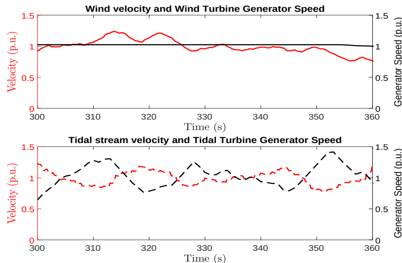
Figure 17. Comparison of generator speed fluctuations in a 10 MW wind turbine and a 110 kW tidal turbine.
