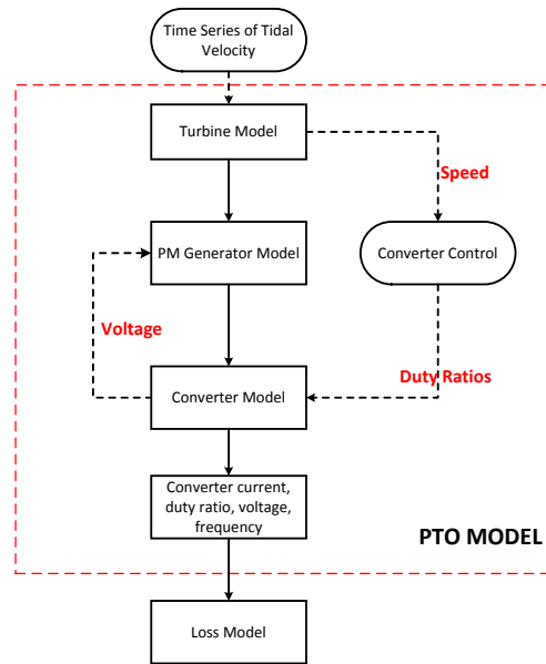
Figure 12. Internal structure of the PTO model.
