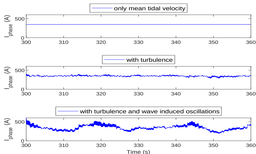
Figure 16. Generator phase currents (RMS values).
