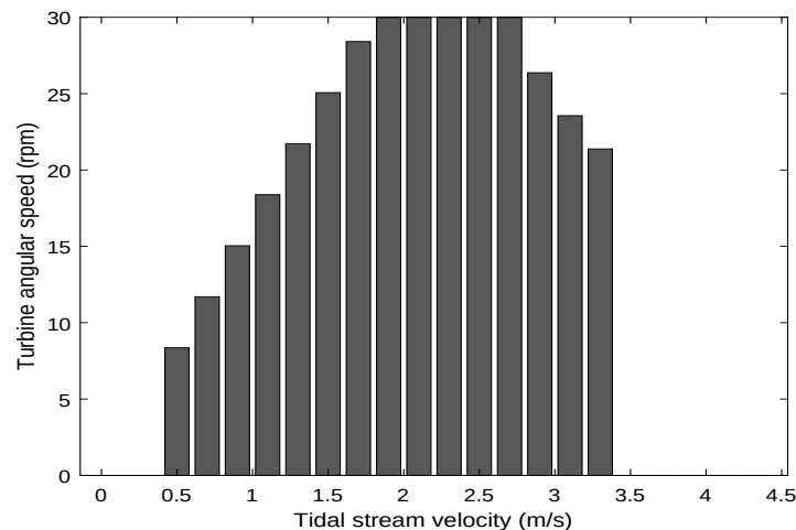
Figure 9. Speed curve of the fixed pitch tidal turbine as a function of the tidal stream velocity.
