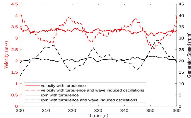
Figure 15. Active speed stall control of Generator speed as a function of change in tidal stream velocity. Mean tidal velocity in this image is set at 3.3 m/s.
