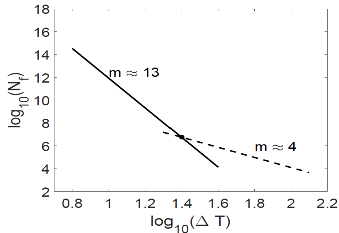
Figure 13. Number of cycles to failure are presented as a function of temperature cycling for a constant mean junction temperature.
