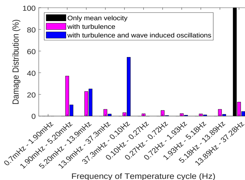
Figure 21. Percentage of total damage vs. frequency of thermal cycling, when turbulence and surface wave ( H_s = 5.75 m, T_p = 11 s) is superimposed to the mean tidal velocity of 2.5 m/s.
