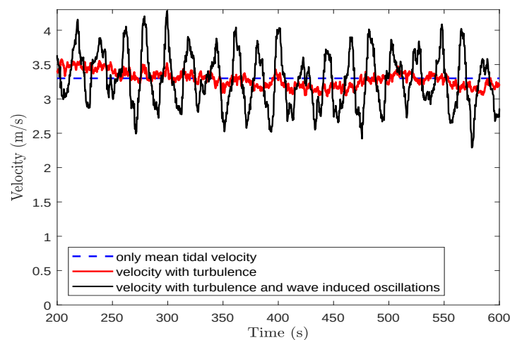
Figure 5. Fluctuations in tidal stream velocity about its mean value (here taken as 3.3 m/s) as a consequence of turbulence and wave induced oscillations.
