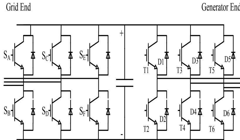
Figure 10. Representative diagram of a 2-level back-to-back voltage source converter (2L-VSC).
