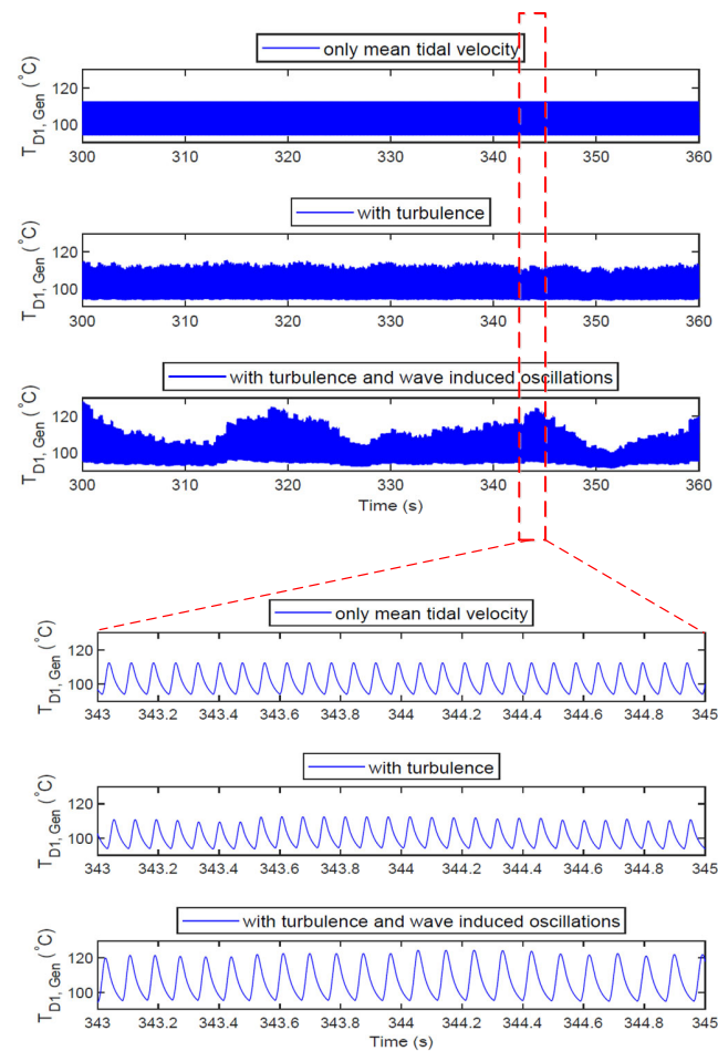
Figure 18. Temperature of the Generator Side Converter Diode (D1) as a function of the fluctuations in the tidal stream velocity.
