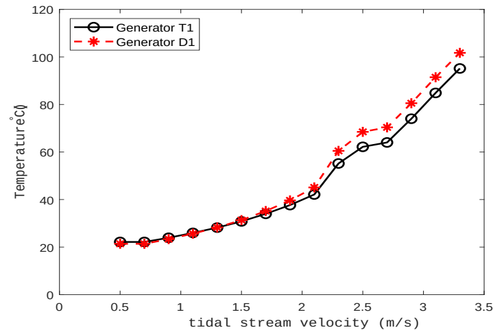
Figure 20. Mean junction temperature of Generator Side Converter Diode.
