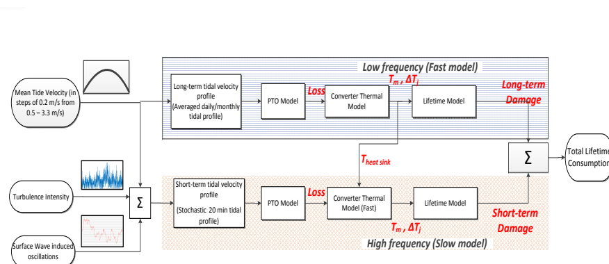
Figure 11. Methodology for lifetime calculations. Finer details of the power take-off (PTO) model are shown in Figure 12.
