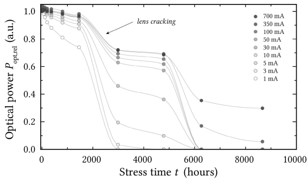
FIGURE 7. Reduction of optical power P_{\text{opt,rel}} for different measurement currents I_m (normalized to the value at 0 h) for a period of 8665 hours. The degradation dynamics are representative for devices stressed at T_j = 100^\circ\text{C} and I_a = 350\text{ mA} .
