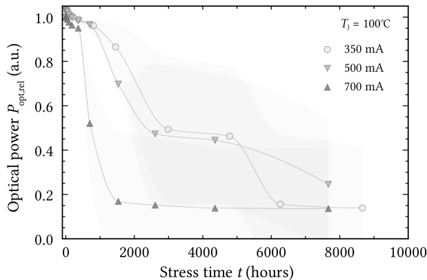
FIGURE 13. Decrease in optical power P_{\text{opt,rel}} measured at I_m = 30 mA for different stress currents I_a = 350 mA, 500 mA and 700 mA at T_j = 100^\circ\text{C} . Mean values with calculated standard deviation (shades).
