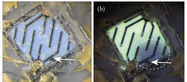
FIGURE 10. Exposed chip surface of damaged device with crack formation. Damage to the ITO layer can be seen in the area of the electrical contacts (a). Identical device at forward-bias with I_m = 350\text{ mA} (b). The area around the defect of the ITO layer shows a significantly lower luminescence.
