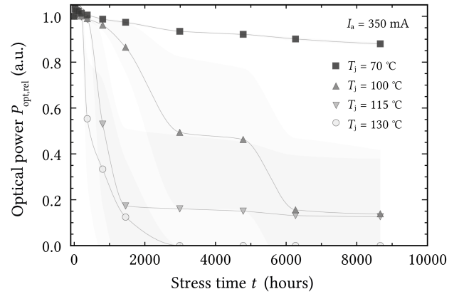
FIGURE 11. Decrease in optical power P_{\text{opt,rel}} measured at I_m = 30 mA for different case temperatures T_j = 70^\circ\text{C} , 100^\circ\text{C} , 115^\circ\text{C} and 130^\circ\text{C} at stress current I_a = 350 mA. Mean values with associated standard deviation (shades).
