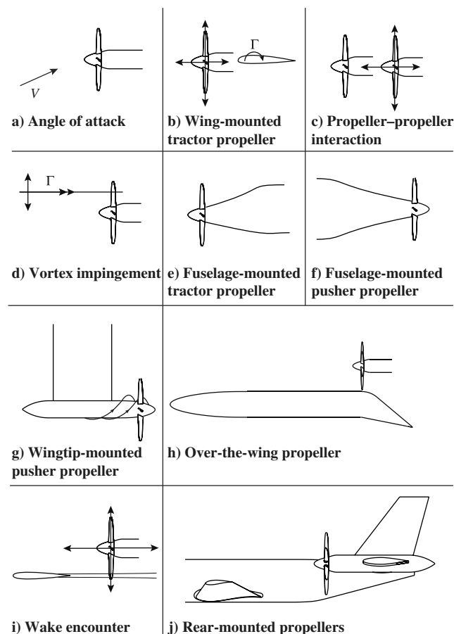
Fig. 1 Typical cases of propellers experiencing nonuniform inflow.
