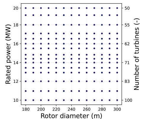
Figure 2. Complete design space showing all the combinations of rated power and rotor diameter.
