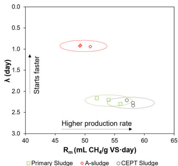
Fig. 5. Correlation between maximum methane production rate ( R_m ) and lag phase ( \lambda ) for each sludge. The three markers for each sludge type indicate triplicate samples. The circle represents 95% confidence level. (For interpretation of the references to color in this figure legend, the reader is referred to the web version of this article.)
