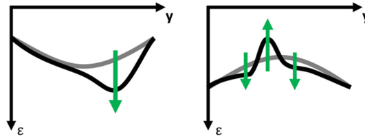
Fig. 2. Graphical representation of the effect of disbond presence on the surface strain of the stiffener foot dependent on the out-of-plane deflection, adapted from [6]. The black line indicates the presence of a disbond and the grey line indicates no disbond presence.
