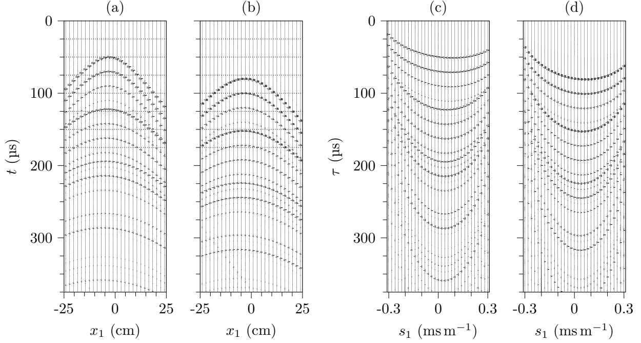
FIG. 5. Downgoing and upgoing wave fields at x_{3,A} = 13 cm. (a) G^+(x_1, x_{3,A}, x_{3,S}, t) * S(t) , (b) G^-(x_1, x_{3,A}, x_{3,S}, t) * S(t) , (c) G^+(s_1, x_{3,A}, x_{3,S}, \tau) * S(\tau) , (d) G^-(s_1, x_{3,A}, x_{3,S}, \tau) * S(\tau) .
