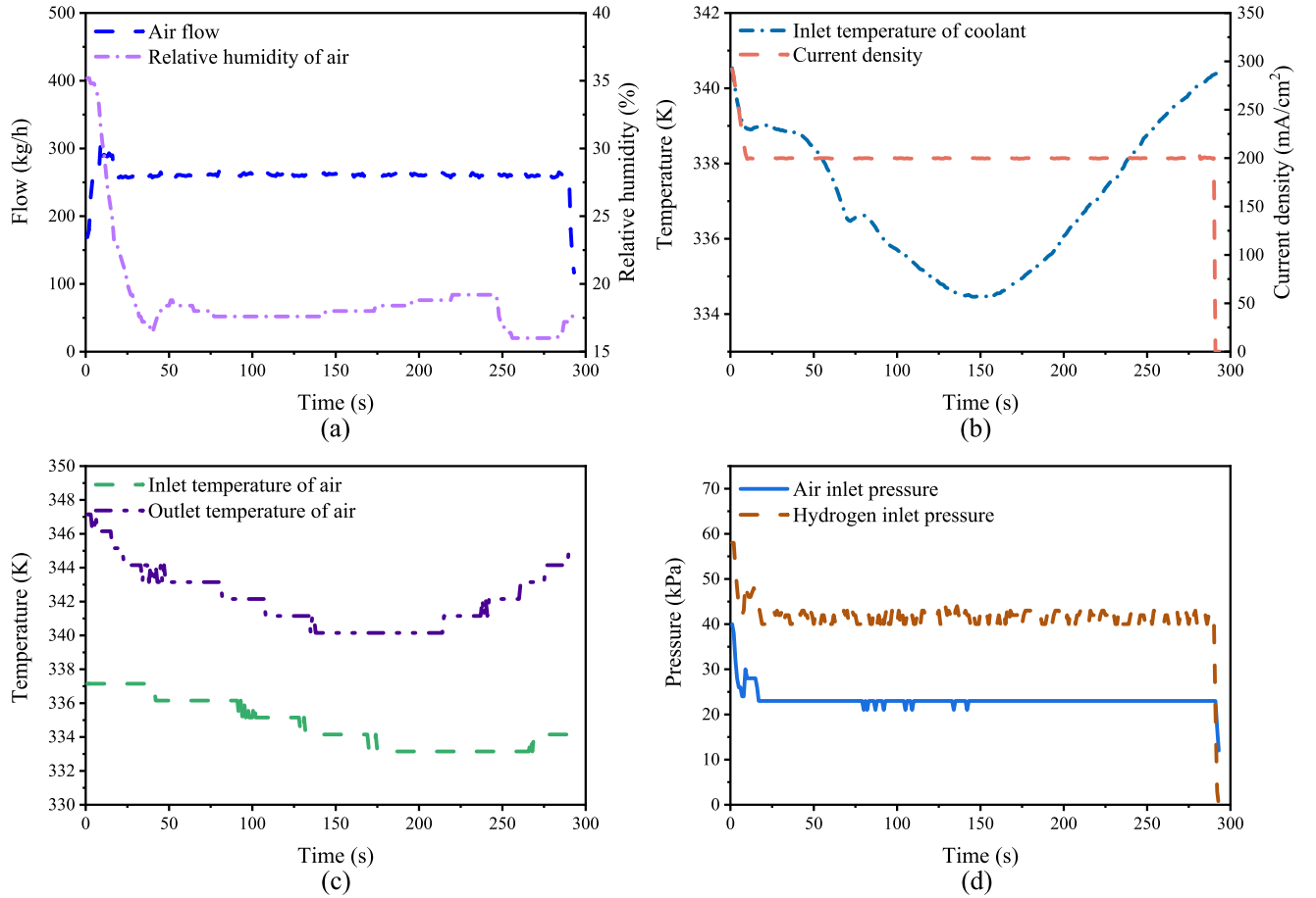
Fig. 2. Main operating parameters during shutdown purge: (a) air flow rate and RH; (b) cooling water inlet temperature and current density; (c) purge air inlet/outlet temperature; and (d) air/hydrogen inlet pressure.
