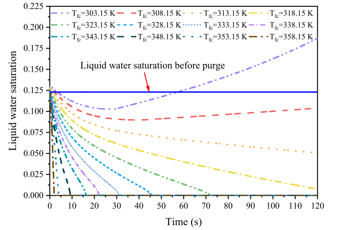
Fig. 9. Purging curves of liquid water on the cathode side at different cell temperatures.
