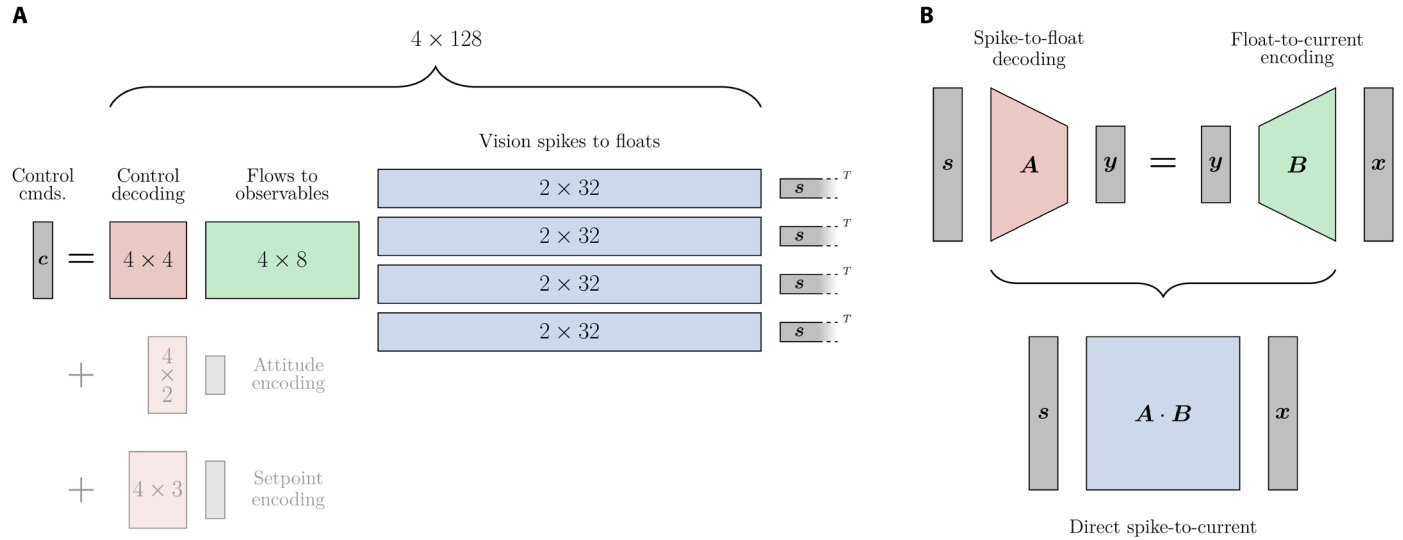
Fig. 7. Merging linear transformations. (A) We go directly from output spikes s of the vision network to control commands c in a single linear decoding by multiplying the involved linear transformation matrices. This is not possible for the matrices used for encoding (shown faded), so we leave these as is. (B) The same principle can be applied to connect two separately trained spiking networks in a spiking manner, from spikes s to currents x , suitable for neuromorphic hardware.
