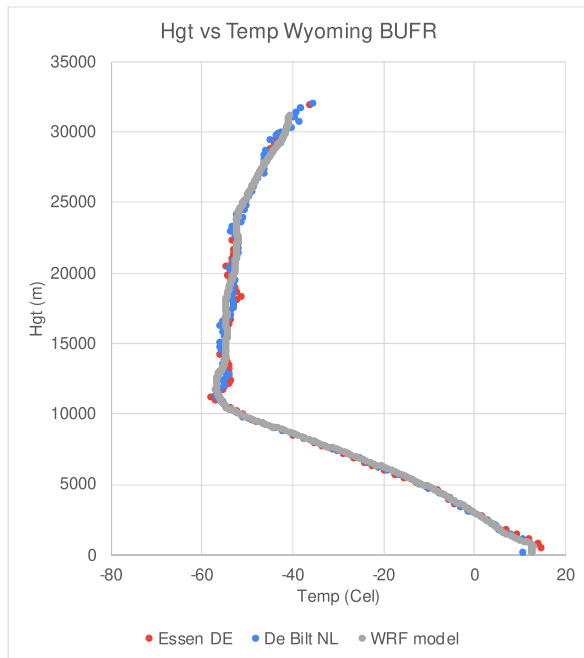
Figure 3 – Relation between temperature and altitude of stations Essen, De Bilt and the WRF model.
