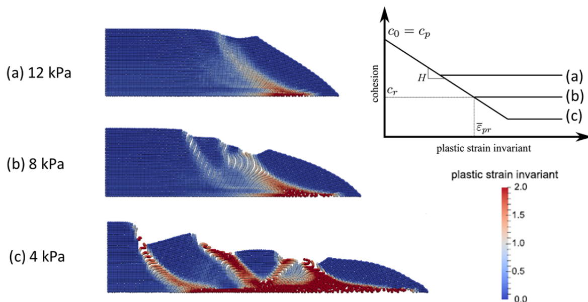
Fig. 3. Final positions of slope failure simulations, with differing residual cohesions.
