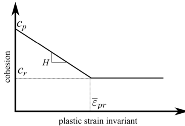
Fig. 1. Schematic of the strain-softening constitutive model [2].
