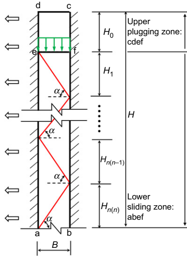
Fig. 4. Calculation model composed of upper plugging zone and lower sliding zone
