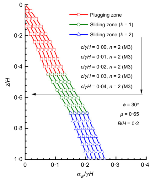
Fig. 14. Effect of normalised soil cohesion on active earth pressure distribution with depth
