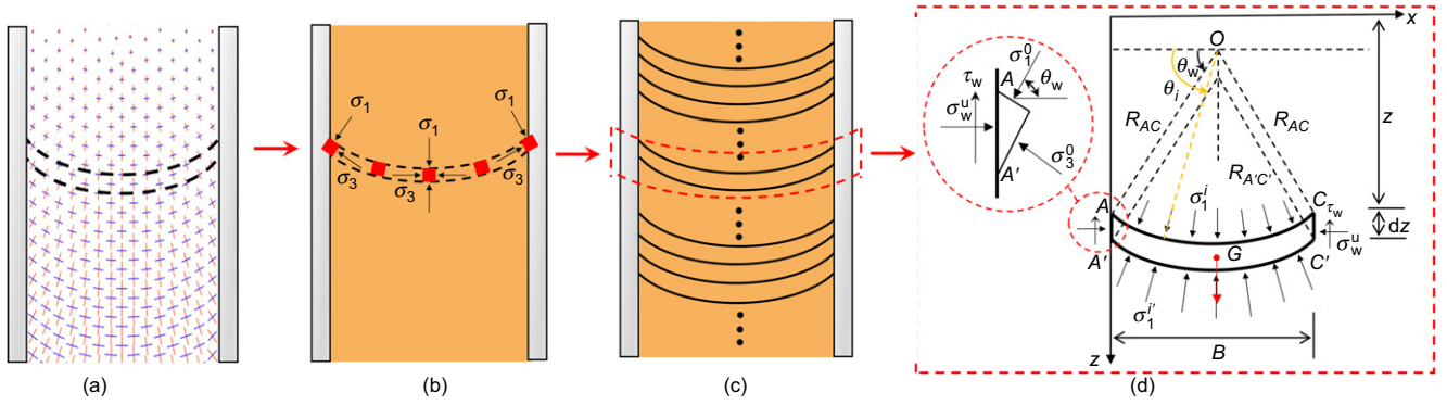
Fig. 5. Calculation model in upper plugging zone: (a) numerical observation principal stress rotation; (b) conceptualisation of arched element along rotation trajectory; (c) discretising narrow soils into arched elements; and (d) force analysis on the arched element
