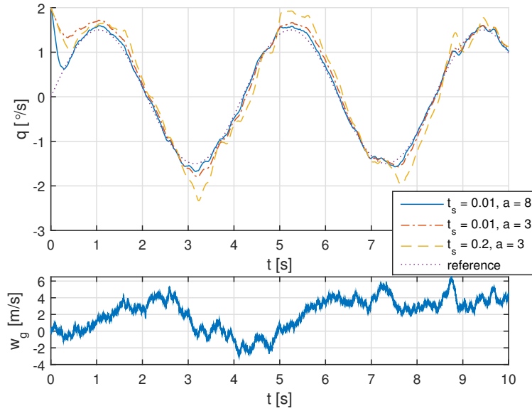
Fig. 2 Pitch rate tracking responses and turbulence input.
