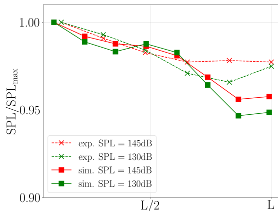
Fig. 12 SPL decay obtained from experiments and simulations with grazing flow, different SPLs and f = 1400 Hz, calculated at the middle of the channel.
