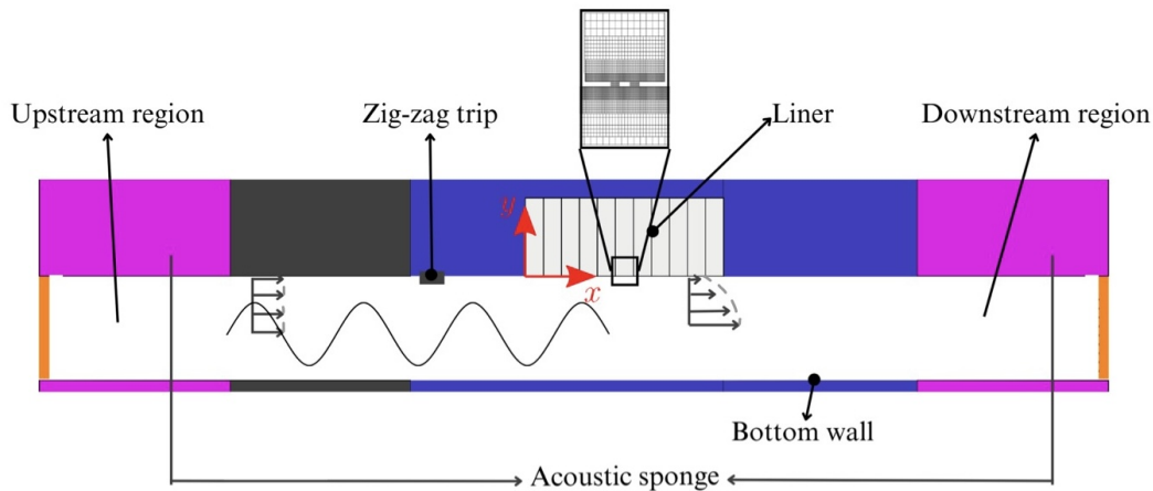
Fig. 3 Full computational domain.
