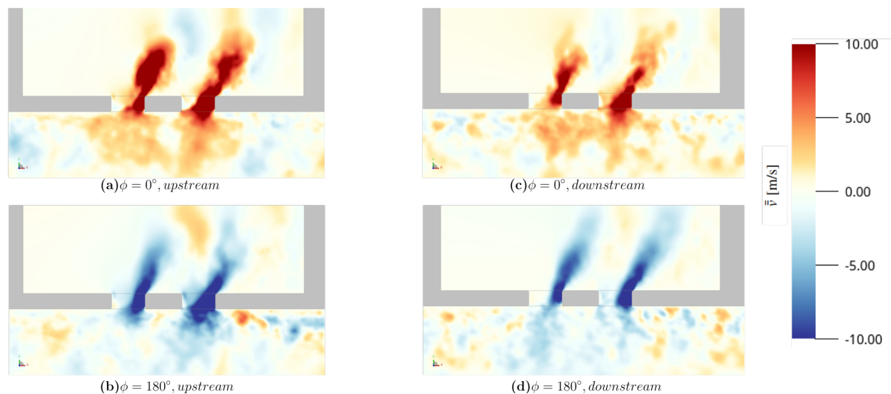
Fig. 18 Contour plot of acoustic-induced vertical velocity \bar{v} for SPL equal to 145 dB, f = 1400 Hz and different acoustic source directions with respect to the grazing flow.
