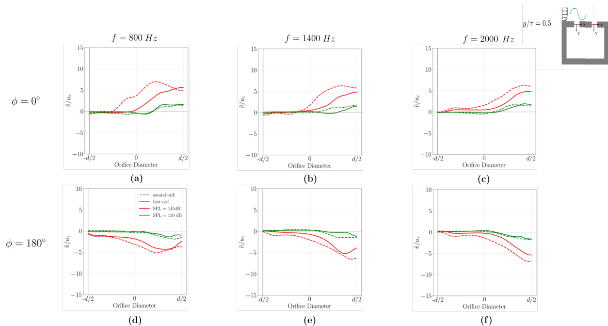
Fig. 14 Spatial distribution along the diameter of the acoustic-induced vertical velocity \bar{v} as a function of the SPL: (a, c) \phi = 0^\circ ; (d, f) \phi = 180^\circ . Acoustic wave with SPL equal to 130dB and 145 dB.
