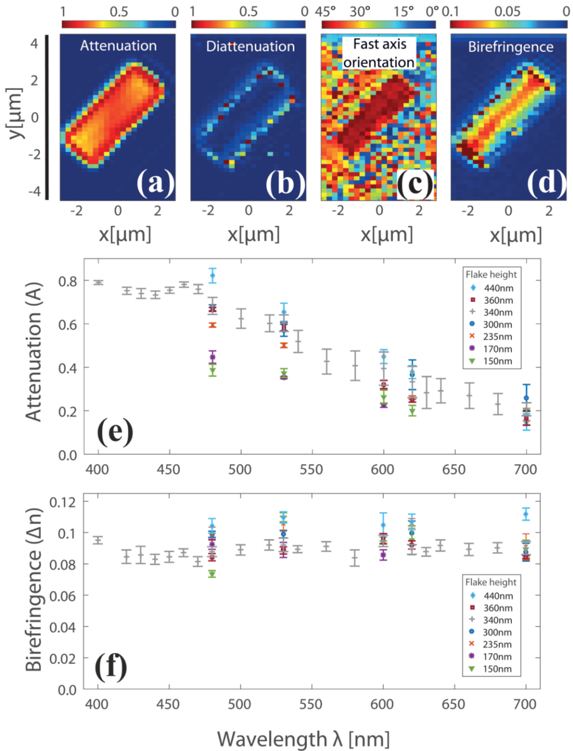
Figure 3 Experimental results. (a-d) Two-dimensional raster scans of a flake of dimensions 5.2 \mu\text{m} \times 2 \mu\text{m} \times 340 \text{ nm} at \lambda = 460 \text{ nm} , showing attenuation, diattenuation, fast axis orientation, and birefringence. The scans were performed as 41 \times 21 steps using a 200 \text{ nm} step size. (e & f) Spectral analysis of attenuation and birefringence for multiple flakes of different heights and lateral dimensions (of at least few microns to avoid edge effects at all wavelengths). The attenuation increases at shorter wavelengths, whereas the birefringence remains high and nearly constant throughout the visible range.
