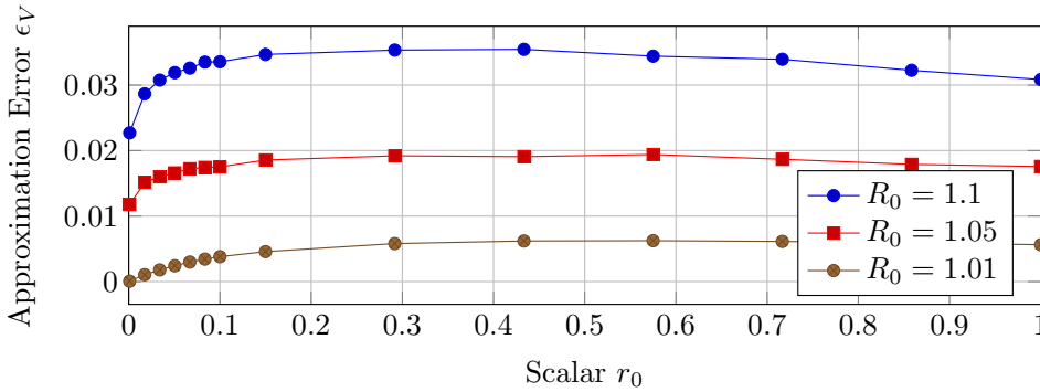
Figure 3.5: Approximation accuracy versus variance of the initial viral state v(0) . The approximation error \epsilon_V versus the scalar r_0 , which controls the variance of the randomly generated initial viral state v(0) , for Barabási-Albert networks with N = 250 nodes.
