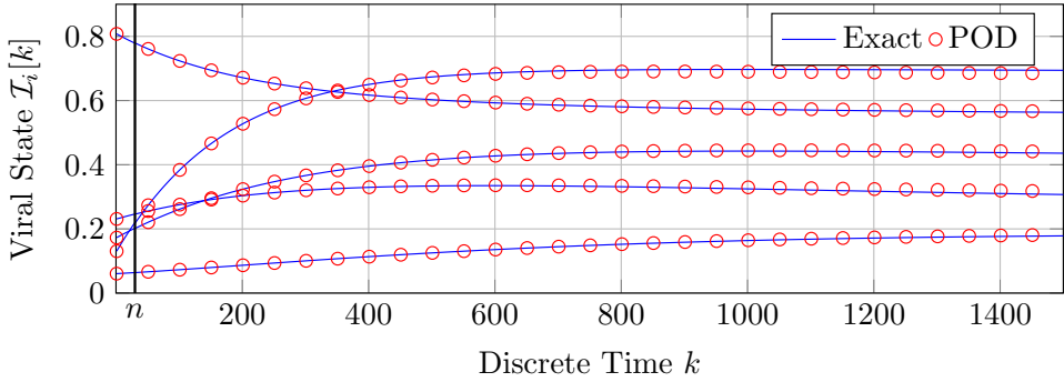
Figure 7.4: Agitation of the viral state dynamics. For a Barabási-Albert random graph with N = 300 nodes and heterogeneous spreading parameters \delta_{\Delta t, i} , \beta_{\Delta t, i j} and a basic reproduction number R_0 = 2 , the exact SIS viral state \mathcal{I}_i[k] in blue and the POD approximation (7.11) in red. For readability, the viral state \mathcal{I}_i[k] of only five nodes is depicted. The approximation equals the linear combination of m = 5 agitation modes y_1, \dots, y_m , which are computed by observing the viral state vector \mathcal{I}[k] until the observation time n = 30 .
