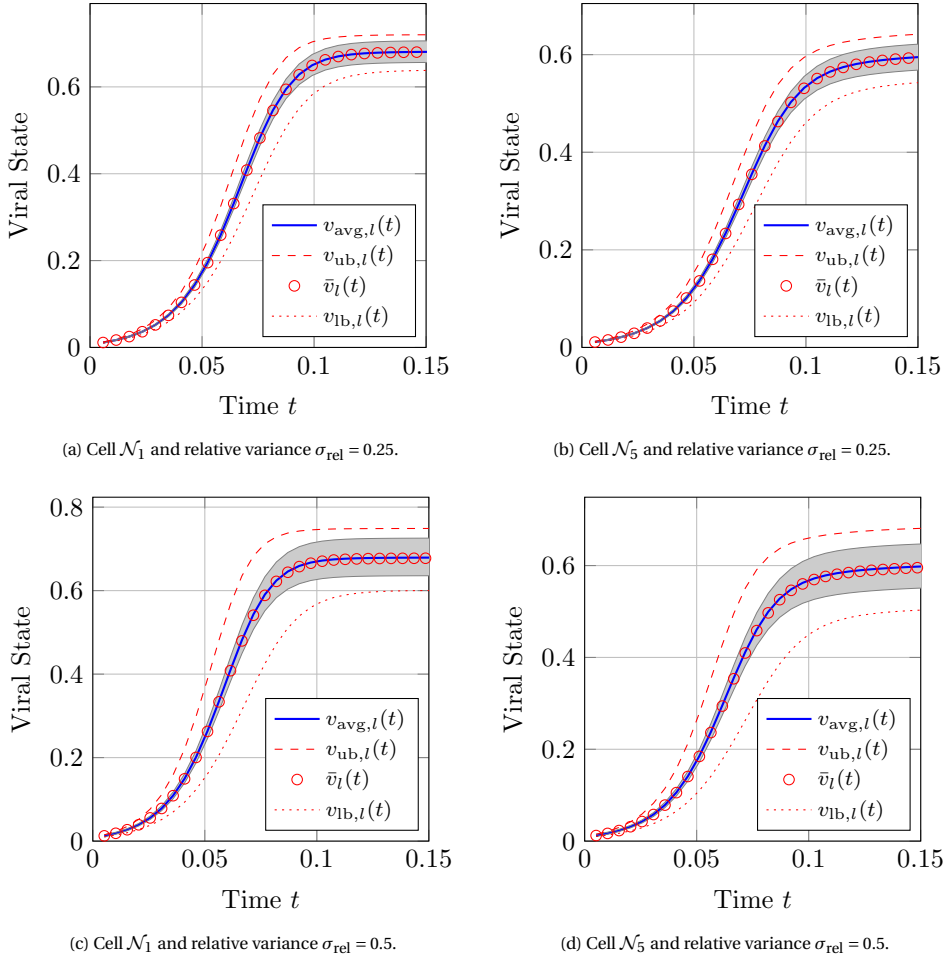
Figure 2.4: Low-dimensional approximation of the viral state dynamics. For a stochastic blockmodel network with N = 1000 nodes and r = 5 cells, the accuracy of the approximation \bar{v}_i(t) and the tightness of the bounds v_{\text{lb},i}(t) , v_{\text{ub},i}(t) are depicted. The reduced-size viral states \bar{v}(t) , v_{\text{lb}}(t) and v_{\text{ub}}(t) equal to the linear combination of m = r = 5 agitation modes y_l , each of which corresponds to one cell. The first and second row correspond to the relative variance \sigma_{\text{rel}} = 0.25 and \sigma_{\text{rel}} = 0.5 , respectively. The left column corresponds to the largest cell \mathcal{N}_1 , the right column corresponds to the smallest cell \mathcal{N}_5 . The viral state v_i(t) of every node i in the respective cell \mathcal{N}_i is within the shaded grey area.
