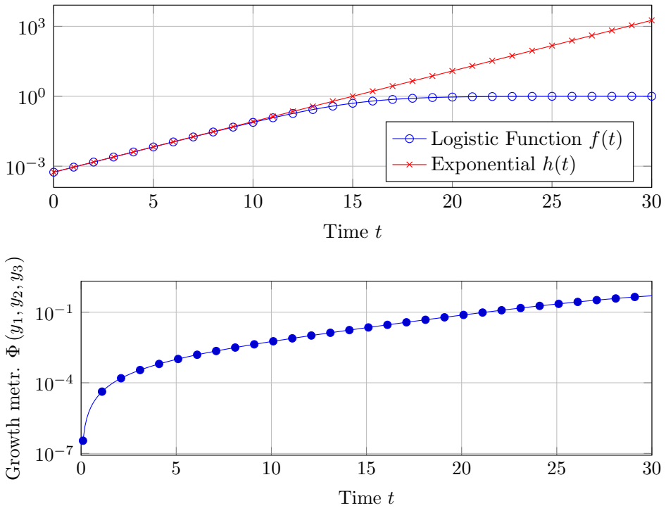
Figure 6.1: Growth metric for a logistic function. Upper subplot: The logistic function f(t) with parameters K = 0.5 , t_0 = 15 and y_\infty = 1 and the exponential function h(t) = y_\infty e^{K(t-t_0)} on a semi-logarithmic scale. Lower subplot: The growth metric \Phi(y_1, y_2, y_3) for the points y_1 = f(0) , y_2 = f(t/2) , y_3 = f(t) versus time t on a semi-logarithmic scale.
