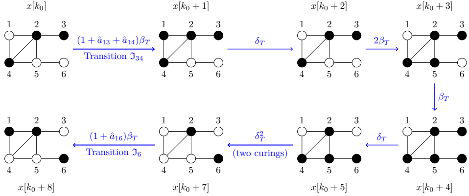
Figure D.1: An illustration of connecting two viral transitions, namely \mathcal{J}_{34} from time k_0 to k_0 + 1 and \mathcal{J}_6 from time k_0 + 7 to k_0 + 8 , for a connected network of six nodes by the procedure described in Subsection D.2.4. Above the blue arrows, the respective transition probabilities are stated. It holds \hat{a}_{12} = a_{12} = 1 and \hat{a}_{ij} = a_{ij} for i, j \geq 2 in the optimisation problem (5.17), and thus the transition probabilities from time k_0 + 1 to k_0 + 7 can be stated without the dependency on \hat{a}_{ij} . On the other hand, both transitions \mathcal{J}_{34} and \mathcal{J}_6 do depend on the elements \hat{a}_{ij} . Since the transition \mathcal{J}_{34} from time k_0 to k_0 + 1 is an infectious transition, we consider that node 1 cures from time k_0 + 1 to k_0 + 2 according to step one in Subsection D.2.4. Then, following the description in step two and three of Subsection D.2.4, every node except node 1 becomes infected from time k_0 + 1 to k_0 + 4 . Subsequently, the nodes 3, 4 and 5 cure from time k_0 + 4 to k_0 + 7 as required for the first state of the transition \mathcal{J}_6 . In Subsection D.2.5, the viral state sequence from time k_0 + 1 to k_0 + 7 is also denoted by \mathfrak{F}(x[k_0 + 1], \mathcal{J}_6) , and its length is given by \tau(\mathfrak{F}(x[k_0 + 1], \mathcal{J}_6)) = 6 .
