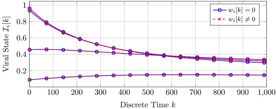
Figure 7.6: SIS dynamics with small model errors. The viral state \mathcal{I}[k] of the discrete-time SIS epidemic model (4.1) for an Erdős-Rényi random graph with N = 20 groups without curing probability control ( \delta_{\max,i} = 0 ), with and without model errors w_i[k] . The viral state \mathcal{I}_i[k] of four of the twenty groups i is depicted.
