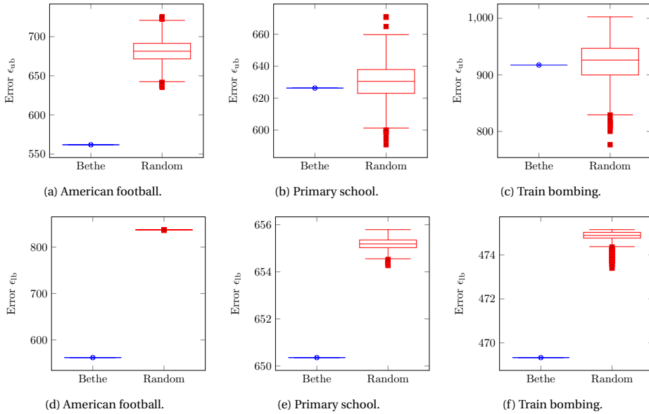
Figure 2.6: Low-dimensional bounds of epidemics on real-world networks. The errors of the low-dimensional bounds \nu_{lb,l}(t) and \nu_{ub,l}(t) , stated by Theorem 2.19, for partitions obtained by Bethe clustering and random partitions. The subplots in the first and second row show the errors \epsilon_{ub} and \epsilon_{lb} of the upper bound \nu_{ub,l}(t) and the lower bound \nu_{ub,l}(t) , respectively.
