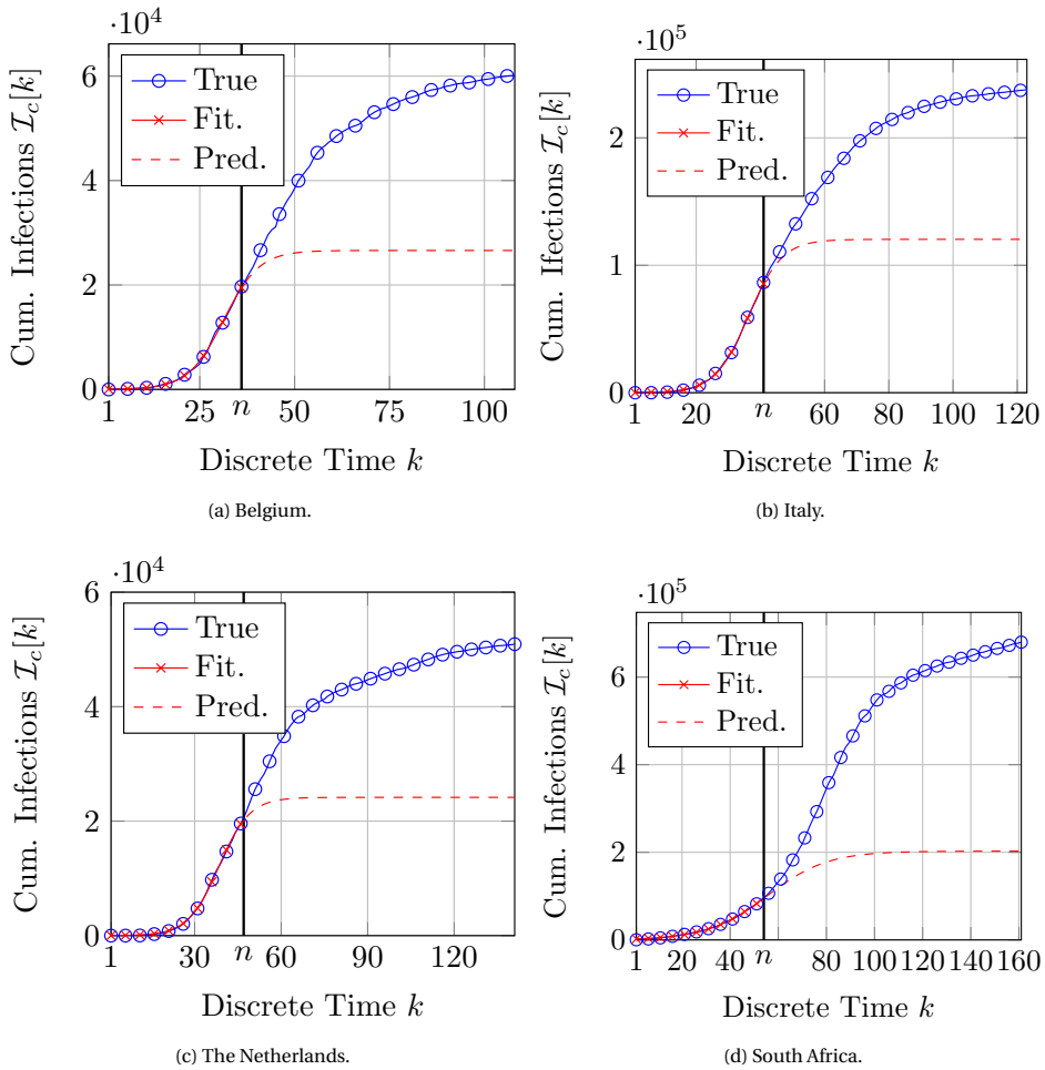
Figure 6.5: Difficulty of predicting COVID-19. The blue curves show the cumulative number of the first wave of confirmed infections with SARS-CoV-2. The red curves shows the logistic curve which is fitted to the infections from day k = 1 until day n and used for predictions at times k > n .
