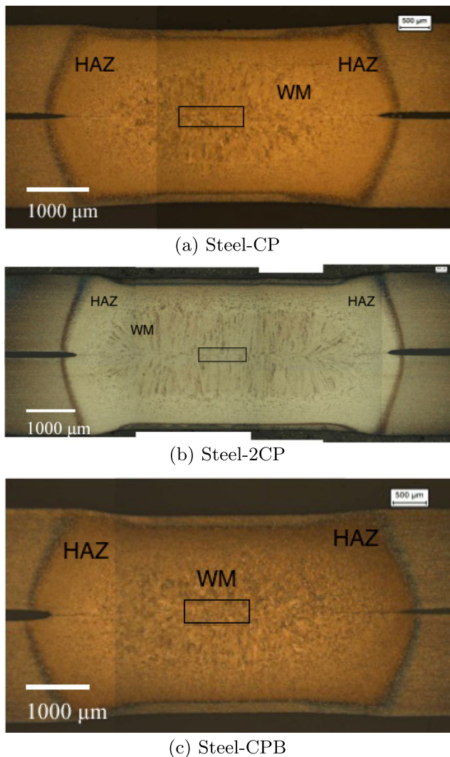
Fig. 10 a–c Overview of the resistance spot welds, where WM is weld metal and HAZ is heat-affected zone. The black box indicates the area where EPMA measurements were carried out. Welds were made at I(min) (see Table 2)
