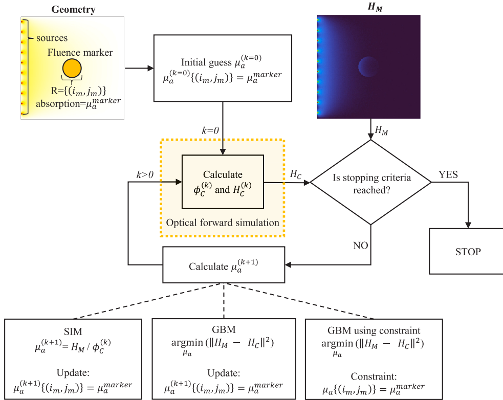
Fig. 1. Fluence marker-based iterative optical inversion for quantitative photoacoustic imaging.
