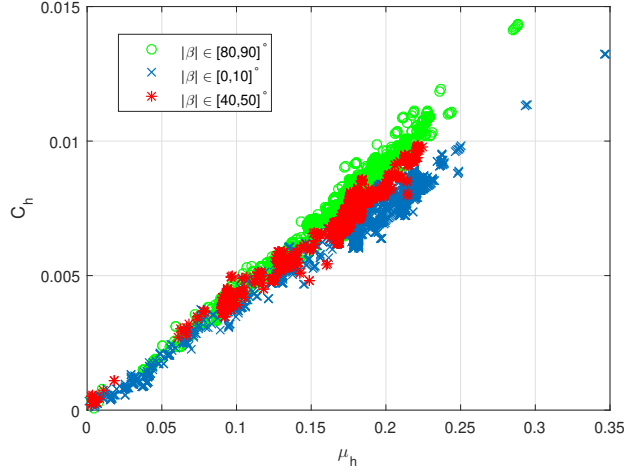
Figure 2.7: C_h vs. \mu_h in different sideslip angle intervals. Plot shows that horizontal force coefficient varies with respect to sideslip angle.
