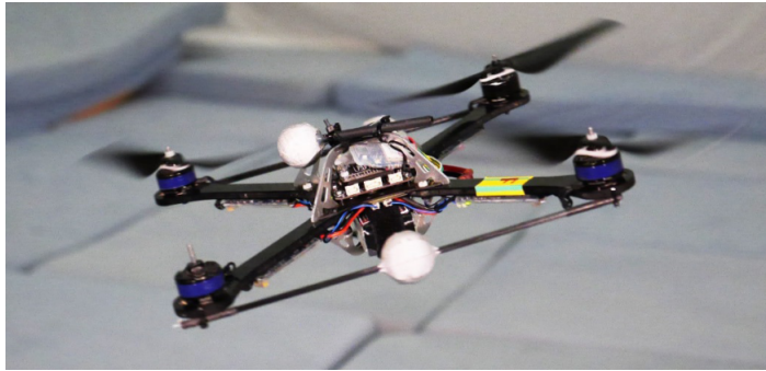
Figure 1.3: Controlled flight of a quadrotor subjected to complete failure of one rotor near hovering condition [25].
