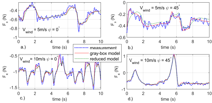
Figure 2.15: Validation results of the F_x model. The gray-box model (red solid line) is compared with the reduced model (green dash-dot). Forward and backward flights are performed for validation. The left two figures show flights with zero heading angle, i.e towards the wind tunnel outlet, while the heading angle is 45^\circ in the right figures.
