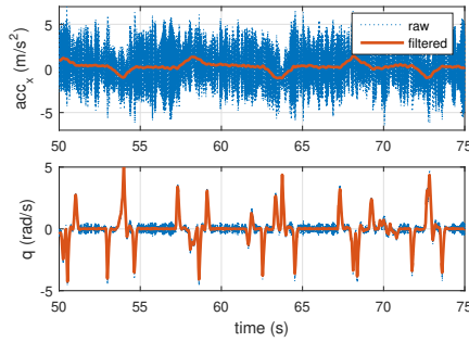
Figure 2.5: Comparison between raw and filtered measurements from accelerometer and gyroscope.
