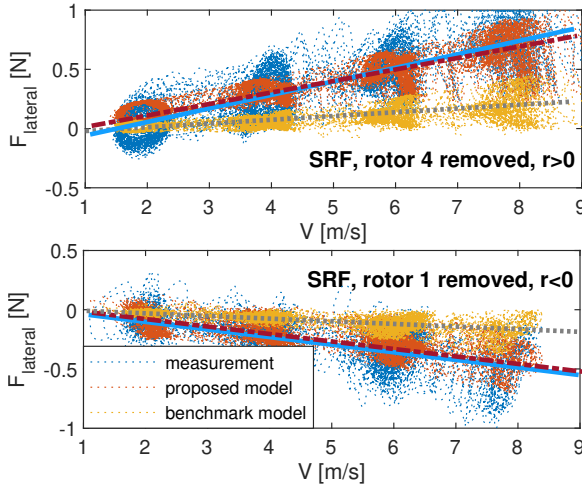
Figure 3.8: Aerodynamic force perpendicular to the air velocity (considered positive to the right with respect to the air velocity). Comparison among the measurement (blue), the proposed model (red) and the benchmark model (yellow), of which trend lines are given in blue-solid, red-dash-dot and gray-dot respectively.
