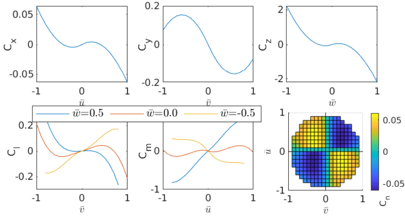
Figure 3.6: The aerodynamic coefficients model of the airframe identified from the flight data.
