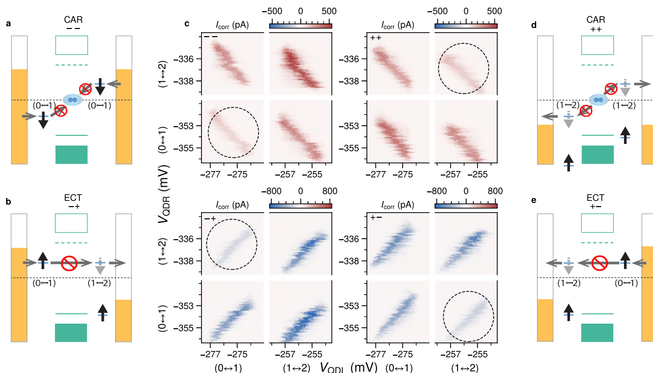
Fig. 3 | Spin blockade at zero magnetic field. Charge stability diagrams are obtained for all four bias polarity combinations, to measure either CAR ( V_L = V_R ) or ECT ( V_L = -V_R ). a , b , d and e show energy diagrams illustrating situations expected to lead to transport blockades. Arrows within the dots either represent an already occupied spin state (black), or a state available to be occupied by an incoming electron (grey). c The corresponding measurements of I_{\text{corr}} plotted against V_{\text{QDL}}
