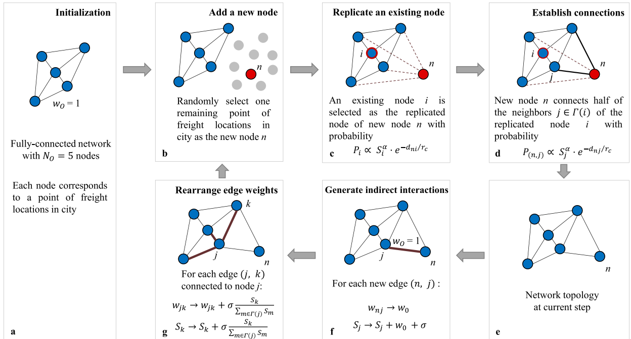
Fig. 3. Model illustration. The growth of network at each step consists of two processes, i.e., topology growth (panel b-d) and weight updates (panel e-g). In the topology growth, a new node n is first added (panel b) and selects its replicated node i (panel c). The neighbors of replicated node i are the potential connecting nodes of the new node n , as indicated as by four dotted lines. d New node n connects to half of the neighbors \Gamma(i) of replicated node i , as indicated as by two bolded solid lines. In weight update process starting from the current topology (panel e), the establishment of a new edge of weight w_0 to the node j generates a total indirect interaction \sigma between new node n and the neighbors of node j (panel f), and \sigma is proportionally distributed among the edges departing from the node j according to the strengths of neighbors \Gamma(j) (panel g).
