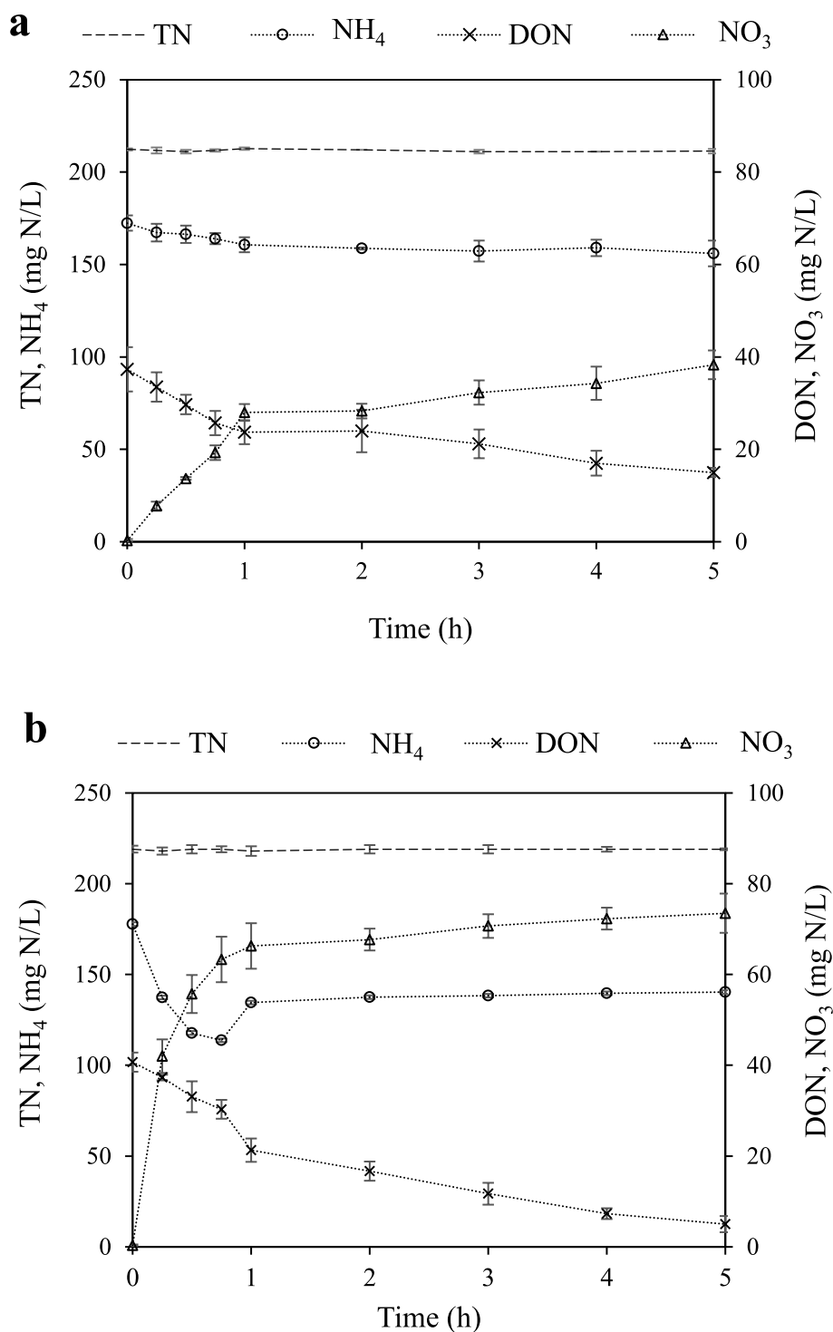
Fig. 5. Oxidation of organic and inorganic nitrogen in digestate supernatant during 5 h (a) O 3 treatment, and (b) O 3 /H 2 O 2 treatment (Initial ozone concentration: 20.5 \pm 0.2 mg/L, ozone flow rate: 51 \pm 2 L/h, sample volume: 2.6 L).
