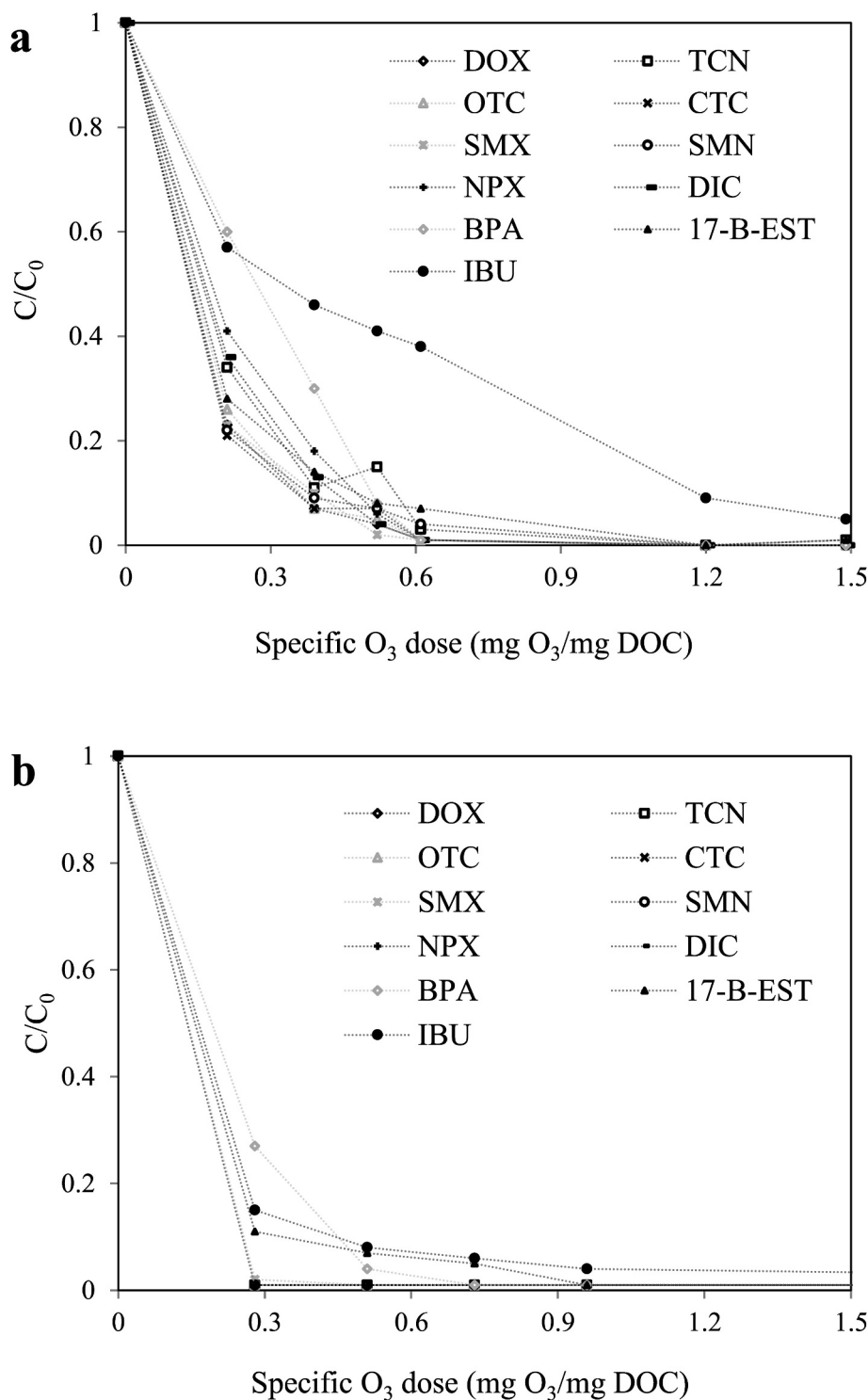
Fig. 4. Removal of various contaminants of emerging concern from digestate supernatant in different specific ozone dose in (a) O 3 and (b), O 3 /H 2 O 2 treatment (H 2 O 2 /O 3 : 2.5) (C 0 and C refers to the initial concentration of each compound and its concentration when a specific O 3 dose was applied within the 5 h experiment).
