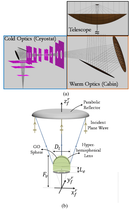
Fig. 1. (a) The GRASP model of the DESHIMA optical system. (b). The equivalent optics used for optimization in reception.
