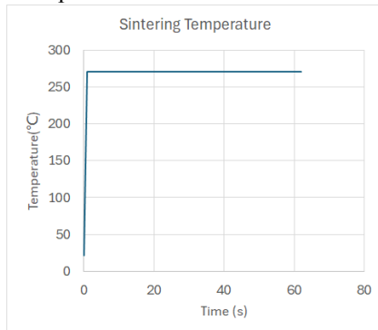
Figure 2 Sintering temperature evolution.
