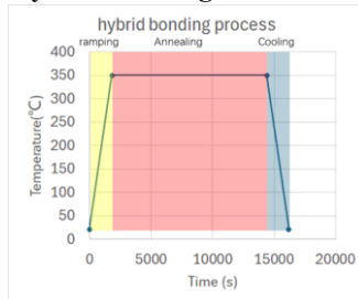
Figure 8 Hybrid bonding temperature profile.
