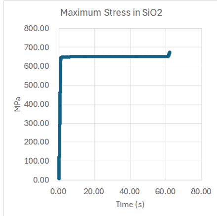
Figure 7 The Maximum Stress of SiO 2 of dielectrics
