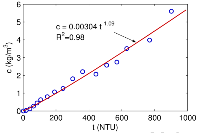
Figure 2. Relationship between OBS-3A measured turbidity ( t ) and suspended sediment concentration ( c ).
