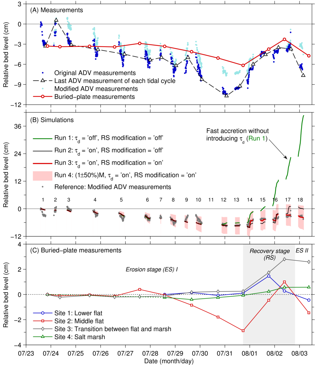
Figure 6. Time series of (A) measured, (B) simulated bed level changes, and (C) buried-plate measurements. To compare with simulated bed level later, ADV measurements are modified with removal the bed level difference between each two measured tidal cycles. ‘RS modification’ in (B) indicates if erosion parameter M and W are modified in the recovery stage.
