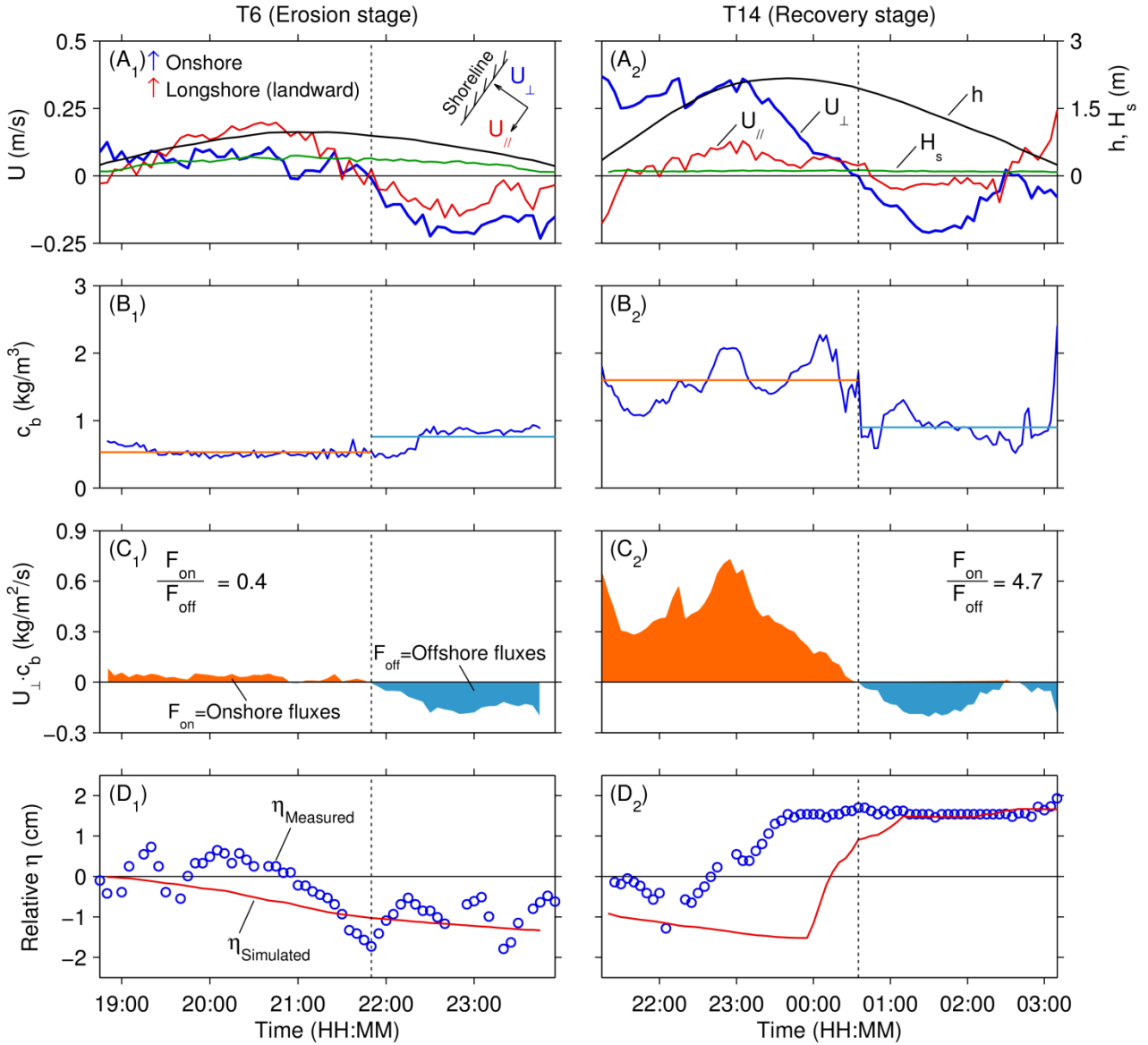
Figure 7. Time series of intra-tidal (A) onshore ( U_{\perp} ) and longshore velocities ( U_{\parallel} ), with water depth ( h ) and significant wave height ( H_s ), (B) Near-bed suspended sediment concentration ( c_b ), (C) Cross-shore near-bed sediment fluxes, and (D) ADV monitored (circle) and simulated (red line) relative bed level ( \eta ) in a typical erosion tidal cycle (T6) and a typical recovery tidal cycle (T14).
