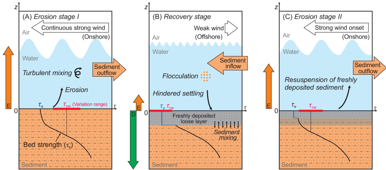
Figure 8. Schematic diagrams illustrate the key processes in three stages. Original vertical distribution of bed strength, representing \tau_e , is redrawn after Winterwerp et al. (2012).
