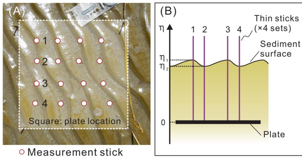
Figure 3. Buried-plate method measures relative bed level change. (A) is the plane view of a real sediment bed showing sticks assignment; transactional view (B) shows sticks are located evenly at ripple crests and troughs.
