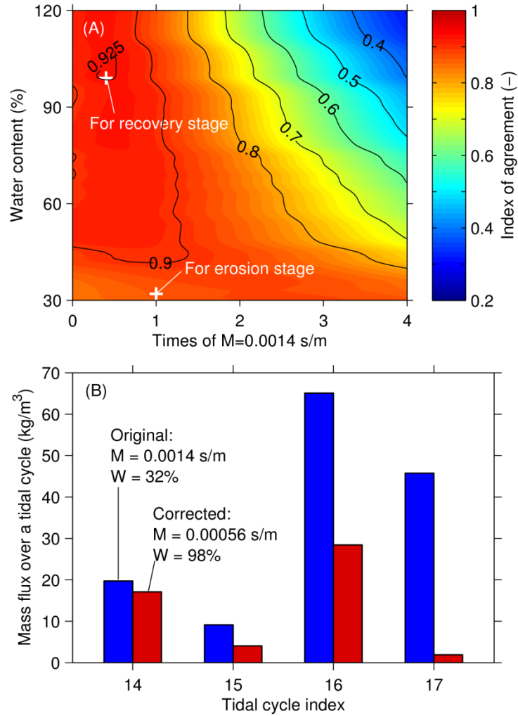
Figure 10. (A) Calibration of erosional parameters M and W for recovery stage. It provides best bed level simulation when M decreases by 60% and W turns from 32% to 98%; (B) Mass fluxes over tidal cycles in recovery stage. Net accreted sediment mass is 2.7 times overestimated without M and W being modified.
