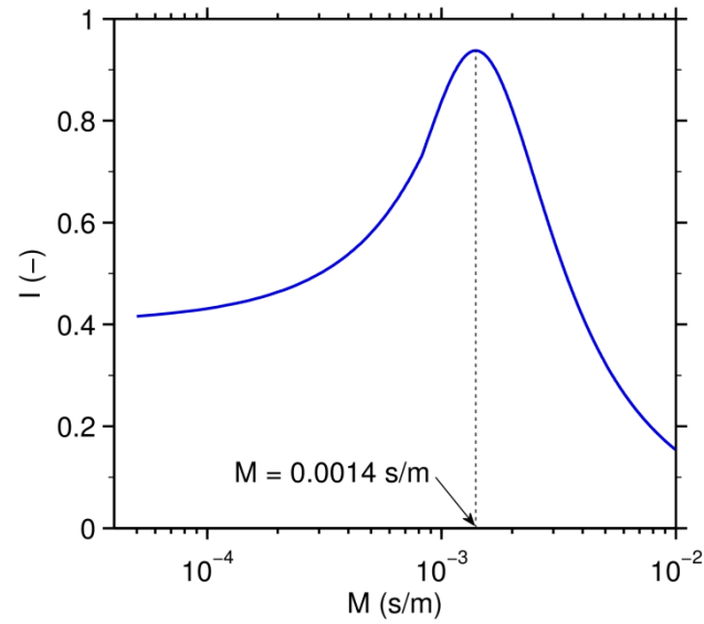
Figure 9. Diagram showing erosion coefficient M in Equation (2) determining the accordance, indicated by index of agreement I , of simulated bed level with ADV measurements. M=0.0014 s/m provides the best estimation in the first erosion stage.
