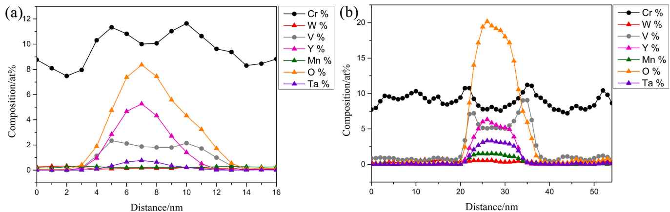
Fig. 6. Composition profiles along the direction of analysis, intercepting a representative particle in (a) ODS Eurofer and (b) ODS Eurofer-2V-1.2Ta.
