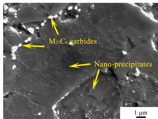
Fig. 1. An SEM micrograph of ODS Eurofer showing M 23 C 6 carbides and nano-precipitates.
