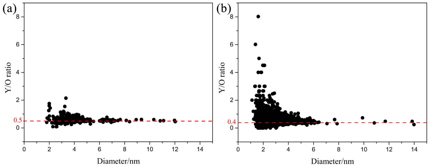
Fig. 5. Y/O ratio of nanoclusters in (a) ODS Eurofer and (b) ODS Eurofer-2V-1.2Ta.
