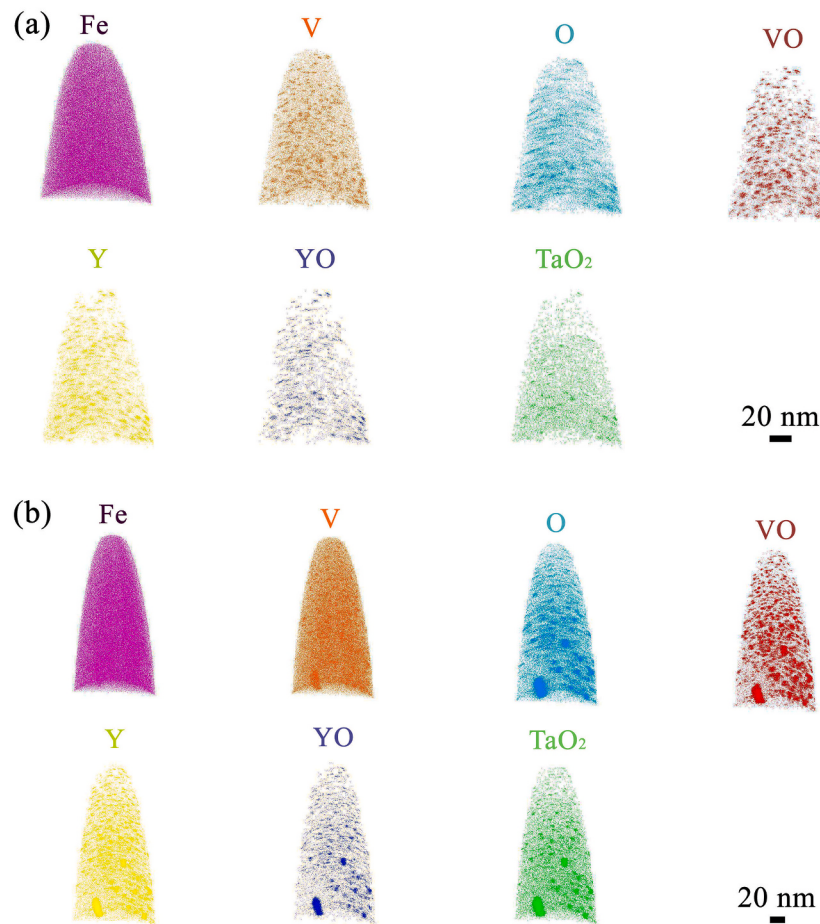
Fig. 3. APT 3D reconstruction of (a) ODS Eurofer and (b) ODS Eurofer-2V-1.2Ta.
