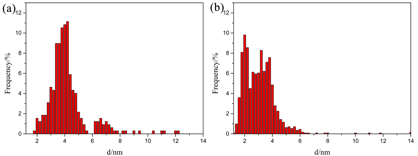
Fig. 4. Size distribution of nanoclusters in (a) ODS Eurofer and (b) ODS Eurofer-2V-1.2Ta.
