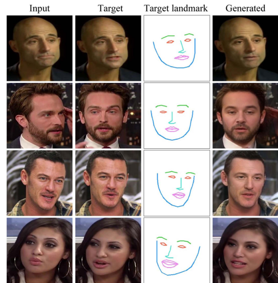
Fig. 8. Generated images based on ground-truth landmarks.
