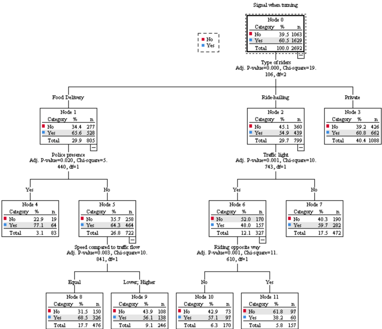
Fig. 5. Classification tree predicting turning signal when making a turn.
