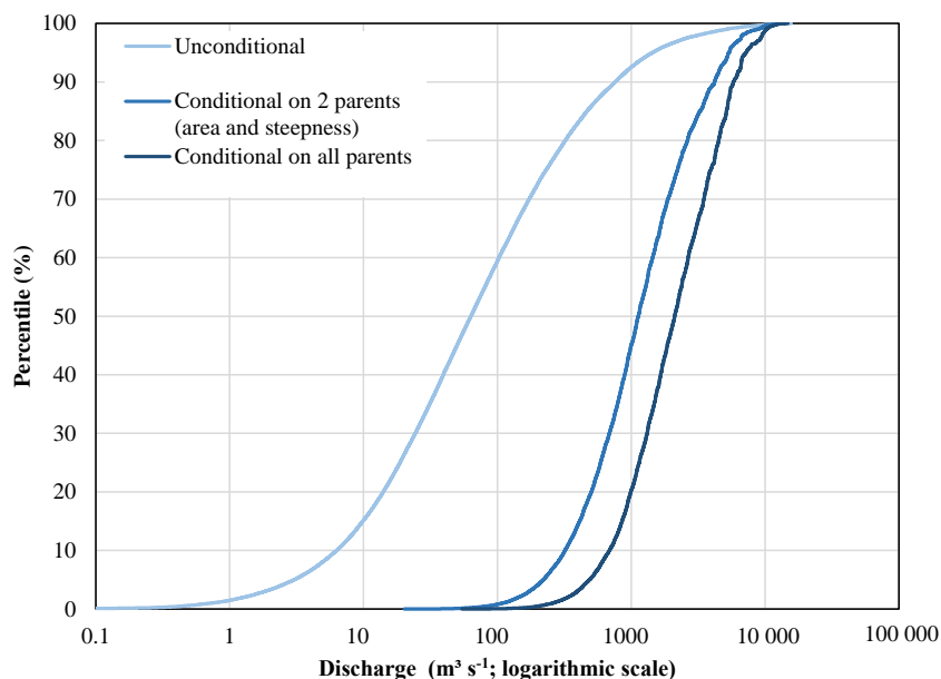
Figure 4. Cumulative probability distribution of river discharge: unconditional and conditionalized on two and seven nodes using values for Basel station in Switzerland (river Rhine, year 2005).
