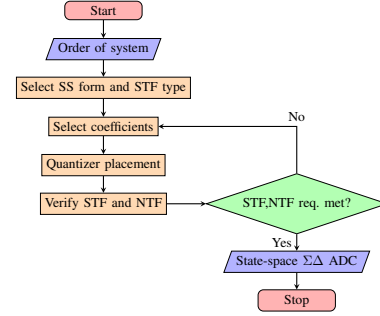
Fig. 1: Flowchart of the state-space based approach for \Sigma\Delta topologies
