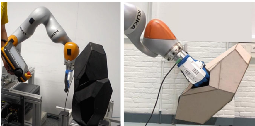
Fig. 3.3 Rhizome 1.0 component mockups and HRI-supported assembly test
