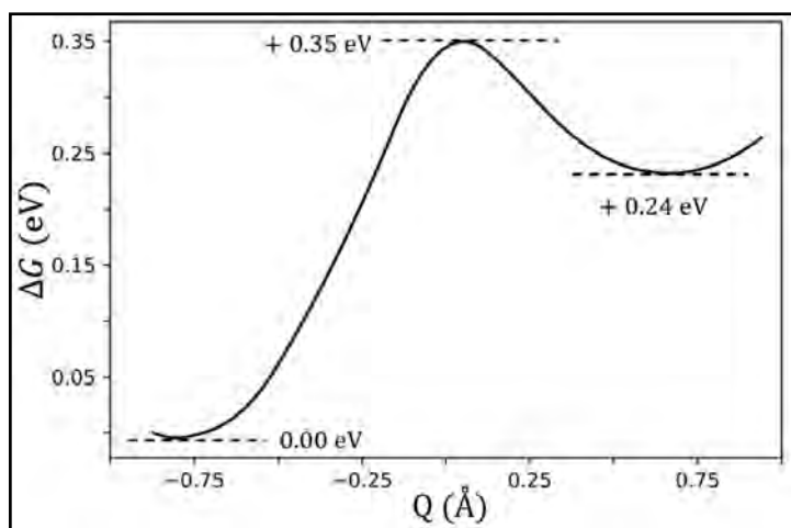
Figure 5. Computed Gibbs free energy profile for deprotonation of \text{H}_2\text{O}^* species using DFT-MD simulations. .
