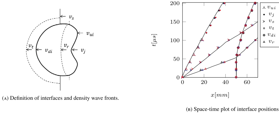
Fig. 14. Shock bubble: definition of interfaces and density wave fronts together with a space time plot of the position of the interfaces and wave fronts. Numerical results (markers) at three grid resolutions: 400x50 ■, 800x100 ■ and 1200x150 ■, compared with Quirk and Karni [58] (solid lines). The maximum Courant number is 0.2.
