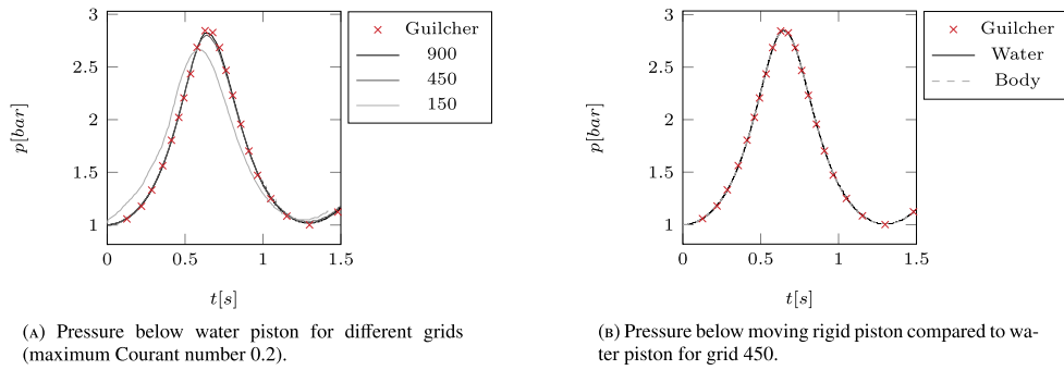
Fig. 12. Piston: pressure below piston as a function of time when piston is either water or moving rigid body.
