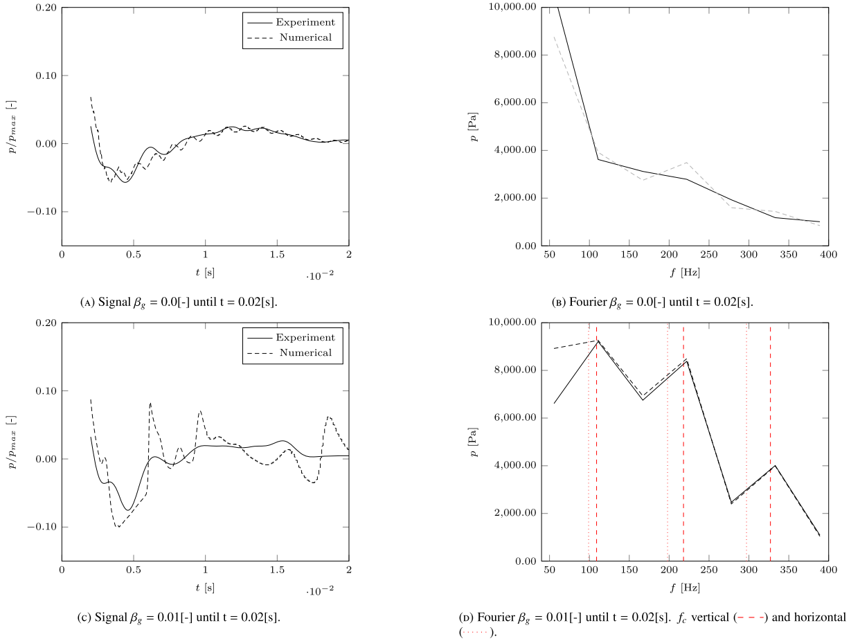
Fig. 25. Filtered time signals and amplitude spectra of post-impact pressure oscillations caused by density waves for \alpha = 15 [deg]. Time signals start 0.002[s] after impact. Band-pass filter between 40 and 400[Hz]). Dashed vertical lines indicate frequencies f_c associated with typical sizes of the domain. The numerical grid used is 109 \times 29 .
