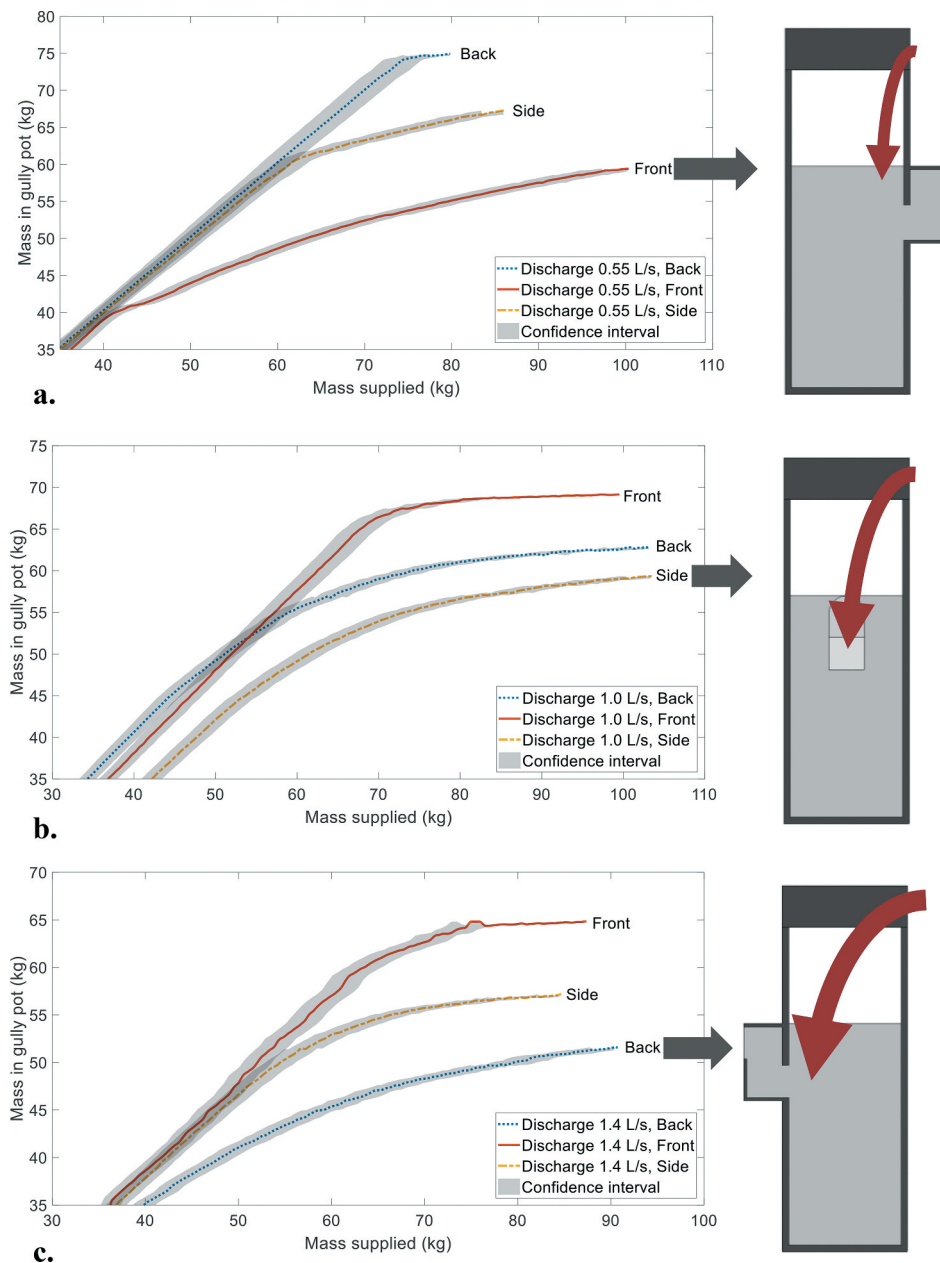
Figure 9. Accumulated mass versus supplied mass for tests with different outlet positions. (a). discharge 0.55 L/s (b). discharge 1.0 L/s c. discharge 1.4 L/s. The drawings at the right indicate for each discharge the outlet position with the lowest removal efficiency.
