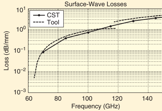
FIGURE 8. Losses associated with the excitation of the first two surface-waves ( \text{TM}_0 and \text{TE}_1 ) for a CPW with w_s = 100 \mu\text{m} , d = 100 \mu\text{m} , H = 500 \mu\text{m} , and \epsilon_r = 11.9 . The result is validated with a full-wave CST simulation.
