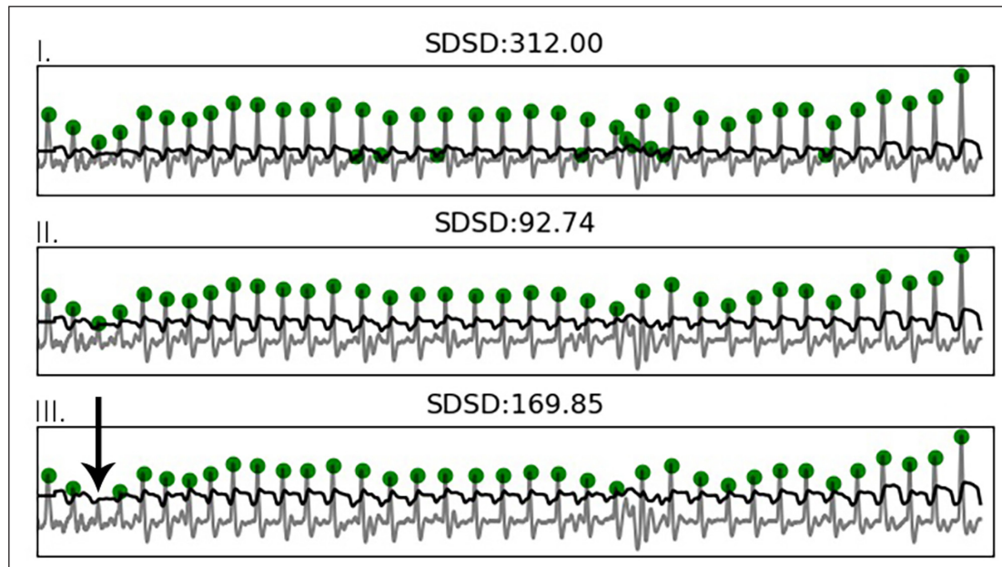
Figure 4: Image showing how the dynamic threshold is fitted using SDSD. The last image (III.) shows that even missing a single beat will lead to a large increase in SDSD compared to the optimal fitting. BPM is also taken into account when fitting.
