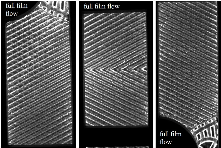
Figure 5.1: Full film flow with G=81 \text{ kgm}^{-2}\text{s}^{-1} and x_{av}=0.30 at the top, middle and bottom windows. The top window is 170 mm(L) \times 86 mm(W) (rectangle) + 80 mm(L) \times 86 mm(W) (triangle). The middle window is 157 mm(L) \times 86 mm(W) (rectangle). The bottom window is 170 mm(L) \times 86 mm(W) (rectangle) + 80 mm(L) \times 86 mm(W) (triangle). The corresponding videos are included in the Appendix of Tao et al. [45].
