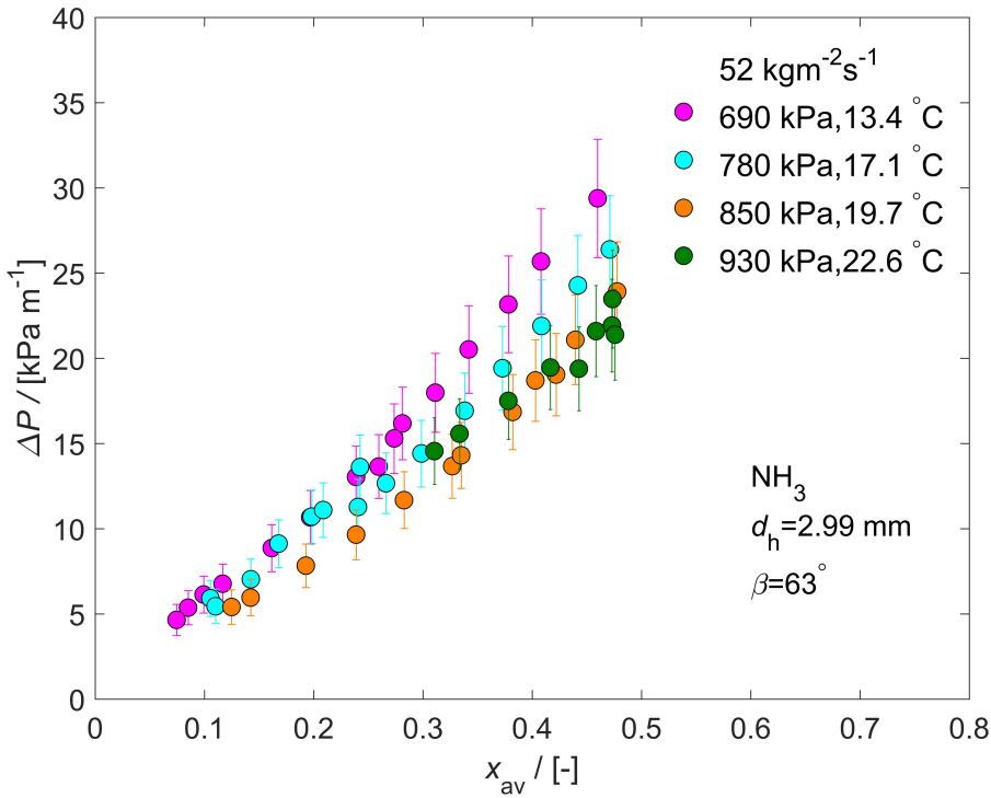
Figure 5.13: Frictional pressure drop with varying averaged vapor quality at different condensation pressure. Frictional pressure drop increases sharply with vapor qualities. Higher condensation pressures reduce frictional pressure drop.
