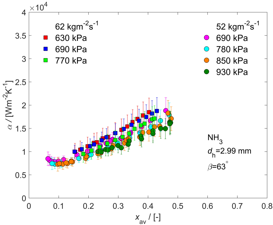
Figure 5.8: Condensation HTC with varying averaged vapor quality at different condensation pressures. HTCs increase sharply with vapor qualities. Higher condensation pressures slightly reduce HTCs.
