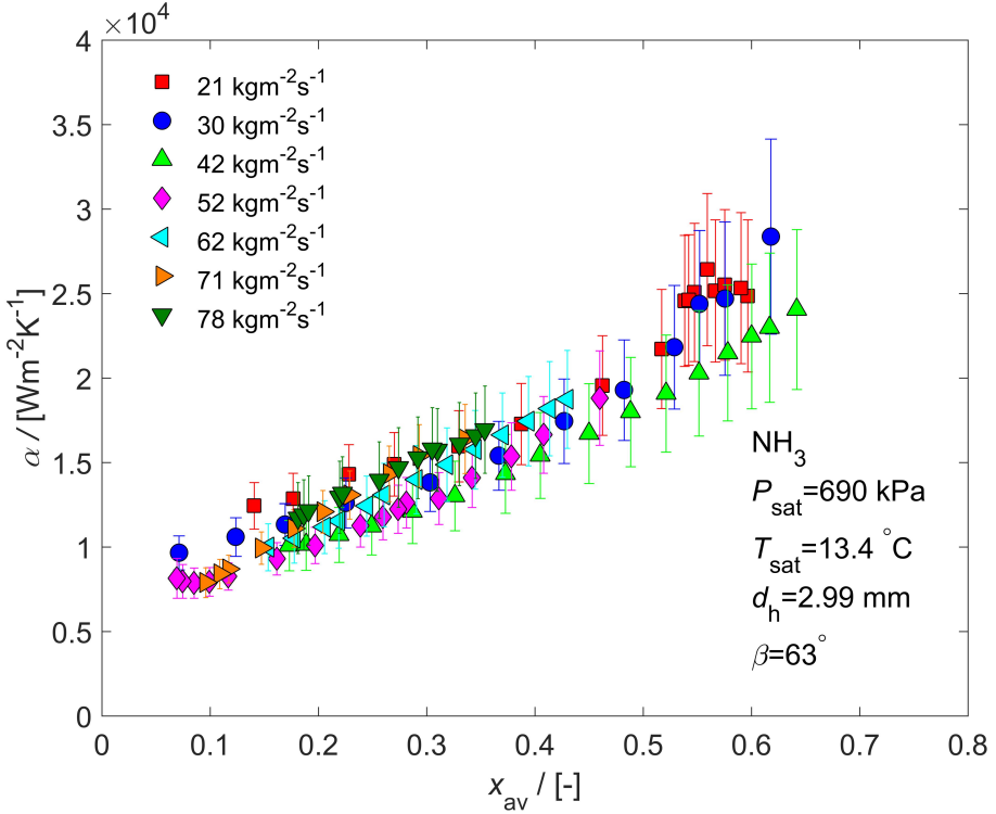
Figure 5.7: Condensation HTC with varying averaged vapor quality at different mass fluxes. HTCs increase significantly with vapor qualities. HTCs decrease slightly with mass fluxes in the range of 21-42 \text{kgm}^{-2}\text{s}^{-1} , and increase moderately from 42 to 78 \text{kgm}^{-2}\text{s}^{-1} .
