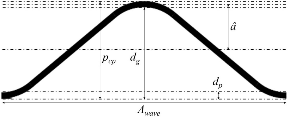
Figure 1.4: The relation between the compressed plate pitch, p_{cp} , the plate thickness, d_p , the channel gap, d_g , the corrugation amplitude, \hat{a} and the corrugation wavelength, \Lambda_{\text{wave}} . Based on Winkelmann [19].
