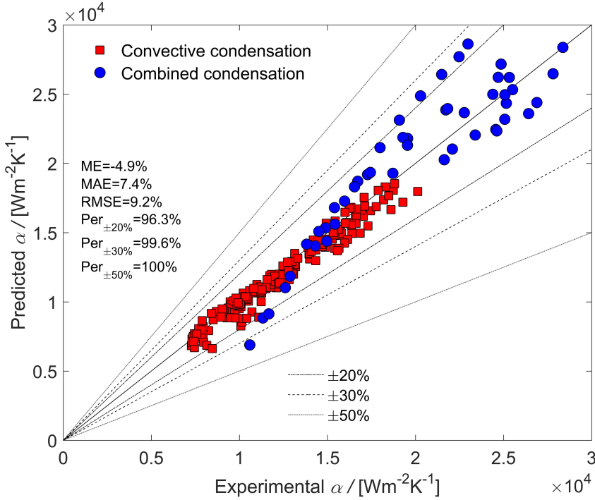
Figure 6.5: Comparison of NH 3 condensation HTC with the proposed model. Mean error (ME): \frac{1}{n} \sum_1^n \frac{\alpha_{pre} - \alpha_{exp}}{\alpha_{exp}} ; Mean absolute error (MAE): \frac{1}{n} \sum_1^n \frac{|\alpha_{pre} - \alpha_{exp}|}{\alpha_{exp}} ; Root mean squared error (RMSE): \sqrt{\frac{1}{n} \sum_1^n \left( \frac{\alpha_{pre} - \alpha_{exp}}{\alpha_{exp}} \right)^2} ; Per_{\pm 20\%} : Percentage of experimental data within \pm 20\% ; Per_{\pm 30\%} : Percentage of experimental data within \pm 30\% ; Per_{\pm 50\%} : Percentage of experimental data within \pm 50\% .
