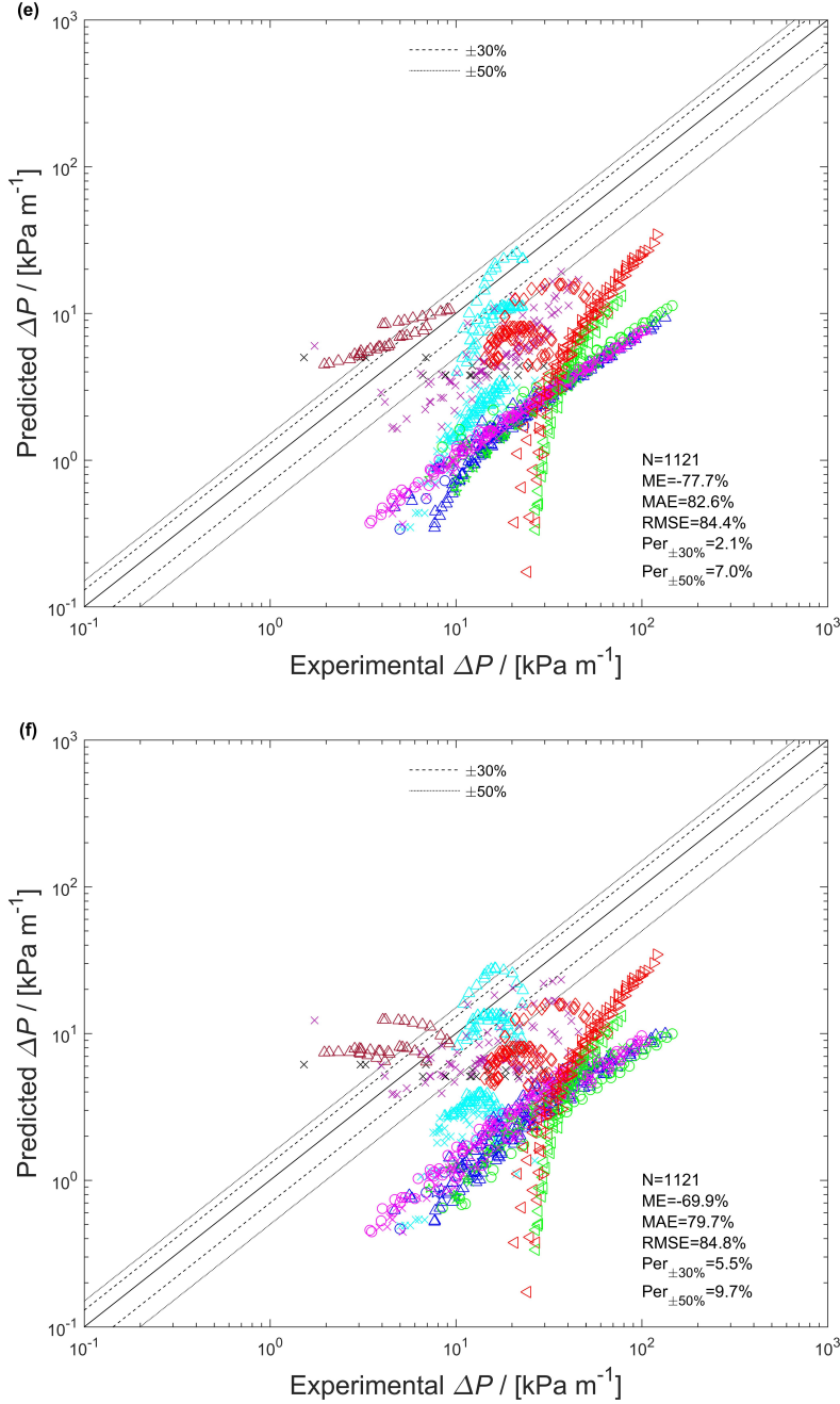
Figure 3.3: Comparison of frictional pressure drop correlations with the experimental data: (a) Kuo et al. [61], (b) Han et al. [87], (c) Hayes et al. [116], (d) Amalfi et al. [53], (e) Winkermann [19], (f) Nilpueng and Wongwises [100]. Number of experimental data (N); Mean error (ME): \frac{1}{n} \sum_1^n \frac{\Delta P_{pre} - \Delta P_{exp}}{\Delta P_{exp}} ; Mean absolute error (MAE): \frac{1}{n} \sum_1^n \frac{|\Delta P_{pre} - \Delta P_{exp}|}{\Delta P_{exp}} ; Root mean squared error (RMSE): \sqrt{\frac{1}{n} \sum_1^n \left( \frac{\Delta P_{pre} - \Delta P_{exp}}{\Delta P_{exp}} \right)^2} ; Per_{\pm 30\%} : Percentage of experimental data within \pm 30\% ; Per_{\pm 50\%} : Percentage of experimental data within \pm 50\% .
