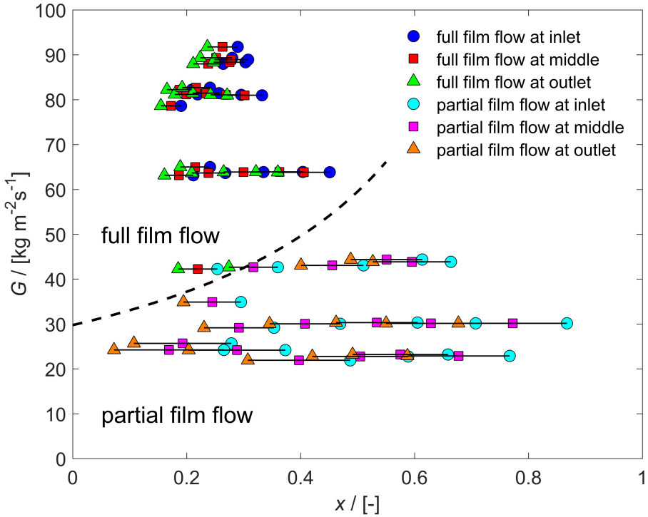
Figure 5.6: Flow pattern map of condensing flow in the PHE, with the vapor quality decreasing from the inlet to the outlet. The flow patterns at the inlet, middle and outlet windows of the same operating condition are connected by lines.
