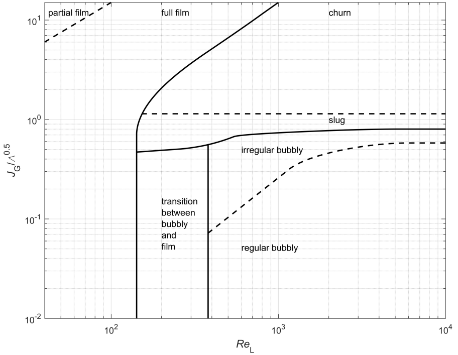
Figure 2.7: Simplified flow pattern map in PHEs using non-dimensional quantities on the x-axis ( Re_L ) and y-axis ( J_G / \Lambda^{0.5} ). The characteristic fluid properties are those of air and water at 25 °C and 150 kPa. Separating lines differentiate regular bubbly flow, irregular bubbly flow, slug flow, churn flow, full film/partial film flow and transition between bubbly and film flow.
