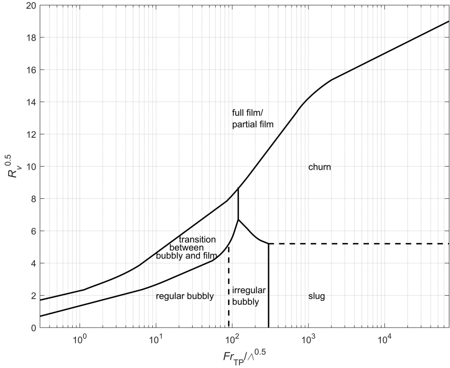
Figure 2.5: Simplified flow pattern map in PHEs, which uses non-dimensional quantities on the x-axis ( Fr_{TP}/\Lambda^{0.5} ) and y-axis ( R_v^{0.5} ). The characteristic fluid properties are these of air and water at 25 °C and 150 kPa. Separating lines differentiate regular bubbly flow, irregular bubbly flow, slug flow, churn flow, full film/partial film flow and transition between bubbly and film flow.
