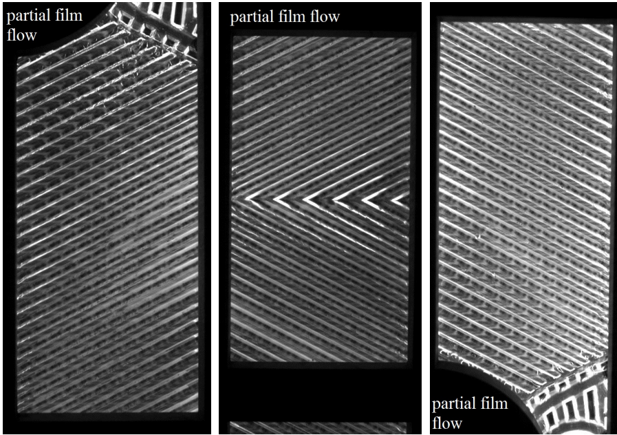
Figure 5.3: Partial film flow with G=43 \text{ kg m}^{-2} \text{ s}^{-1} and x_{av}=0.46 at the top, middle and bottom windows. The top window is 170 \text{ mm(L)} \times 86 \text{ mm(W)} (rectangle) + 80 \text{ mm(L)} \times 86 \text{ mm(W)} (triangle). The middle window is 157 \text{ mm(L)} \times 86 \text{ mm(W)} (rectangle). The bottom window is 170 \text{ mm(L)} \times 86 \text{ mm(W)} (rectangle) + 80 \text{ mm(L)} \times 86 \text{ mm(W)} (triangle). The corresponding videos are included in the Appendix of Tao et al. [45].
