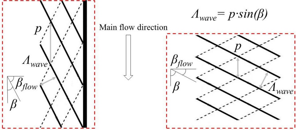
Figure 1.3: Representation of the corrugation profile including the corrugation pitch, p , the corrugation wavelength, \Lambda_{\text{wave}} , and the chevron angle, \beta ; \beta_{\text{flow}} is the angle of the corrugation perpendicular to the flow direction; (left) small chevron angle and (right) large chevron angle. Based on Winkelmann [19].
