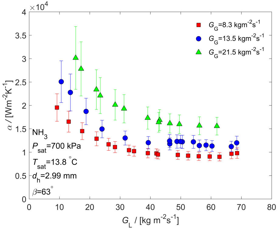
Figure 5.9: Condensation HTC with varying liquid and vapor mass fluxes. HTCs decrease with increasing liquid mass fluxes at small values, and stay almost constant at larger values. Larger vapor mass fluxes increase the HTCs.
