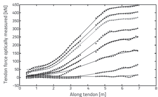
Figure 5. Load distribution along tendon as measured by Brillouin optical time domain analysis [18]
