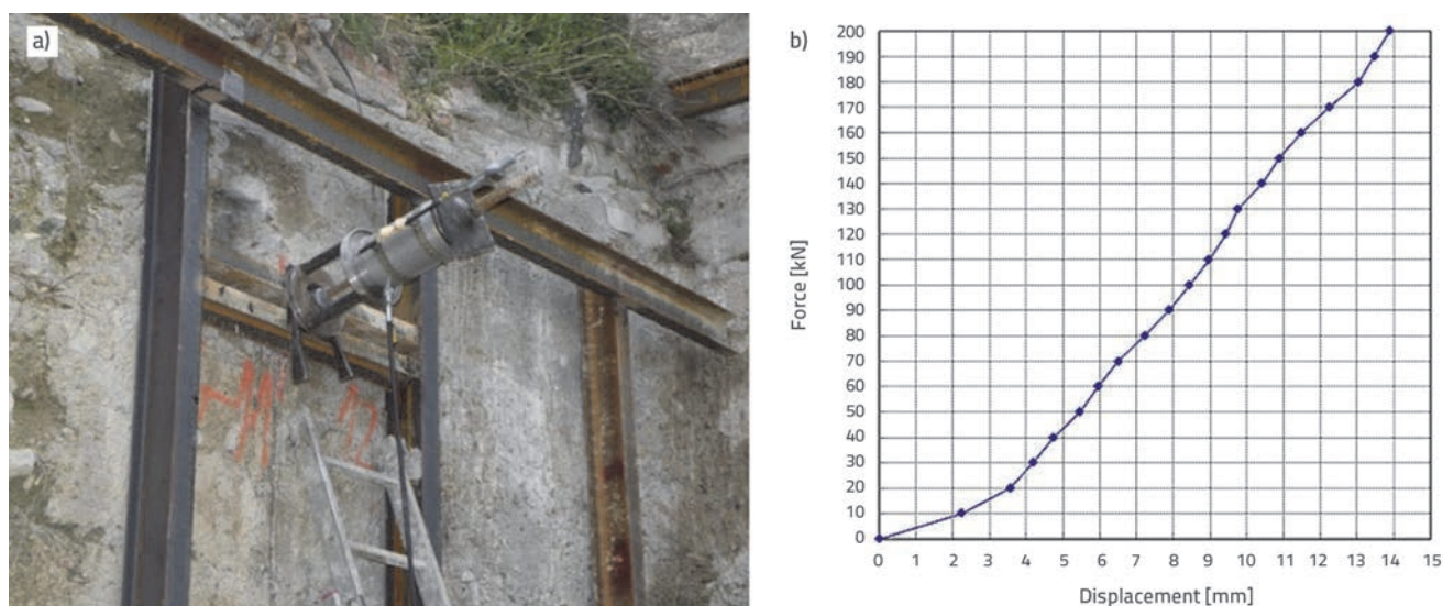
Figure 2. a) pull-out test in progress, b) resulting force-displacement graph of so-called proof load test; test location: foundation pit in Split, Croatia [8]
