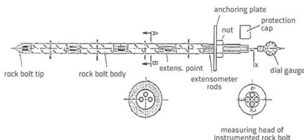
Figure 4. Elements of a measuring rock bolt, modified from [12]
