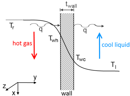
Figure 3-4: Regenerative cooling heat transfer mechanism (xy view)
