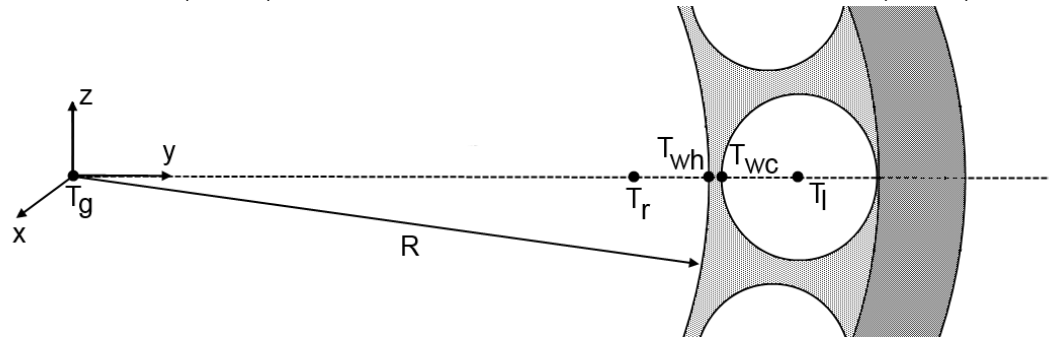
Figure 3-6: Cross section thrust chamber/nozzle with cooling channels (yz view)
