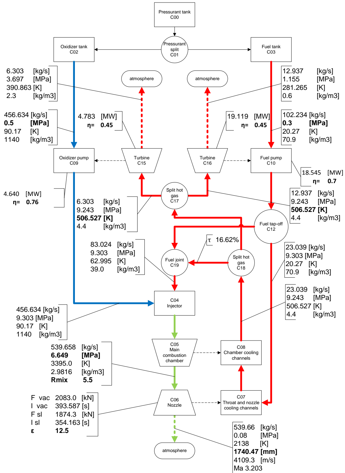
Figure 7-1: Thermodynamic conditions inside expander bleed cycle engine SE-21D calculated with LiRA R.R.L. Ernst
