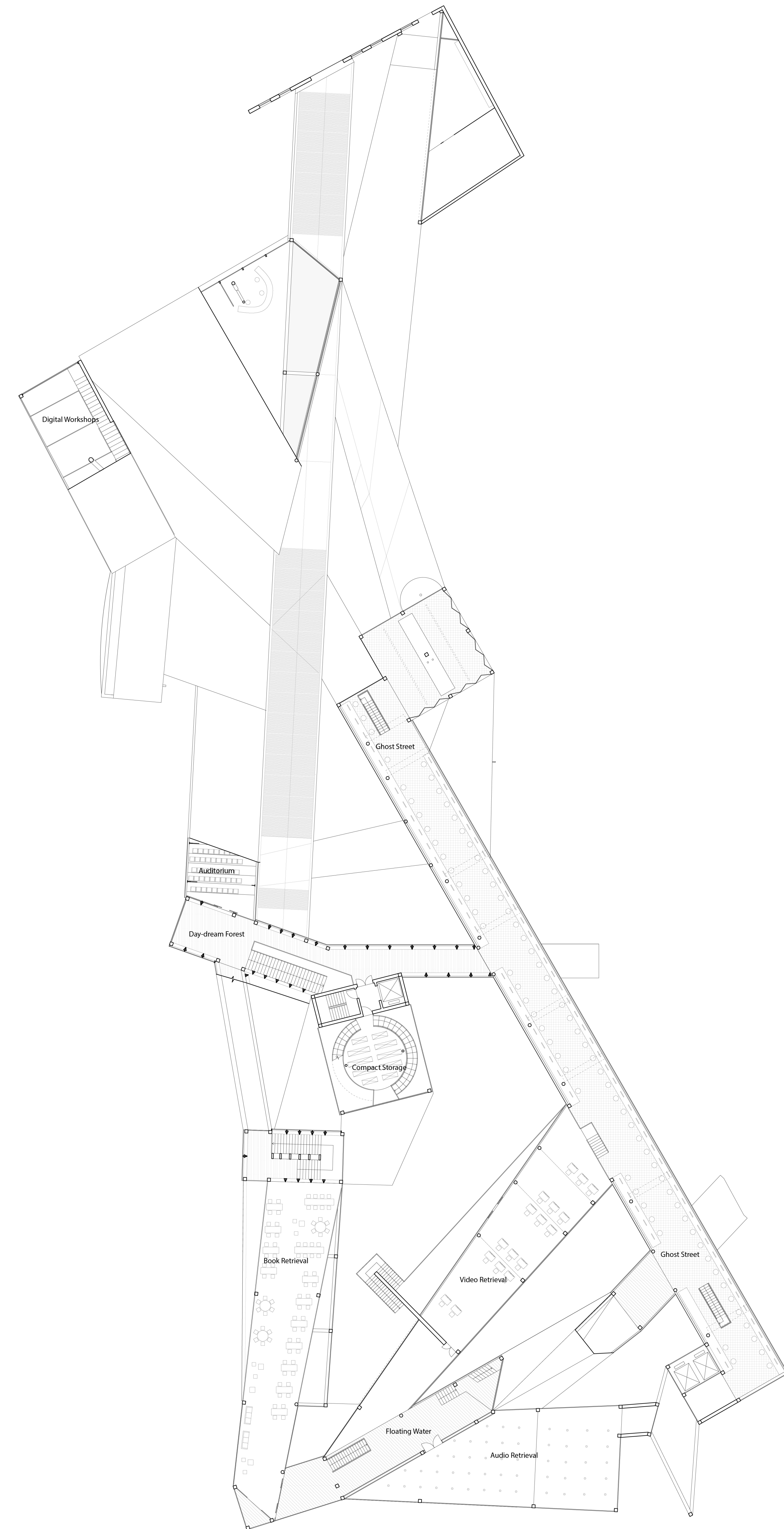
1st Floor Plan 1:200
