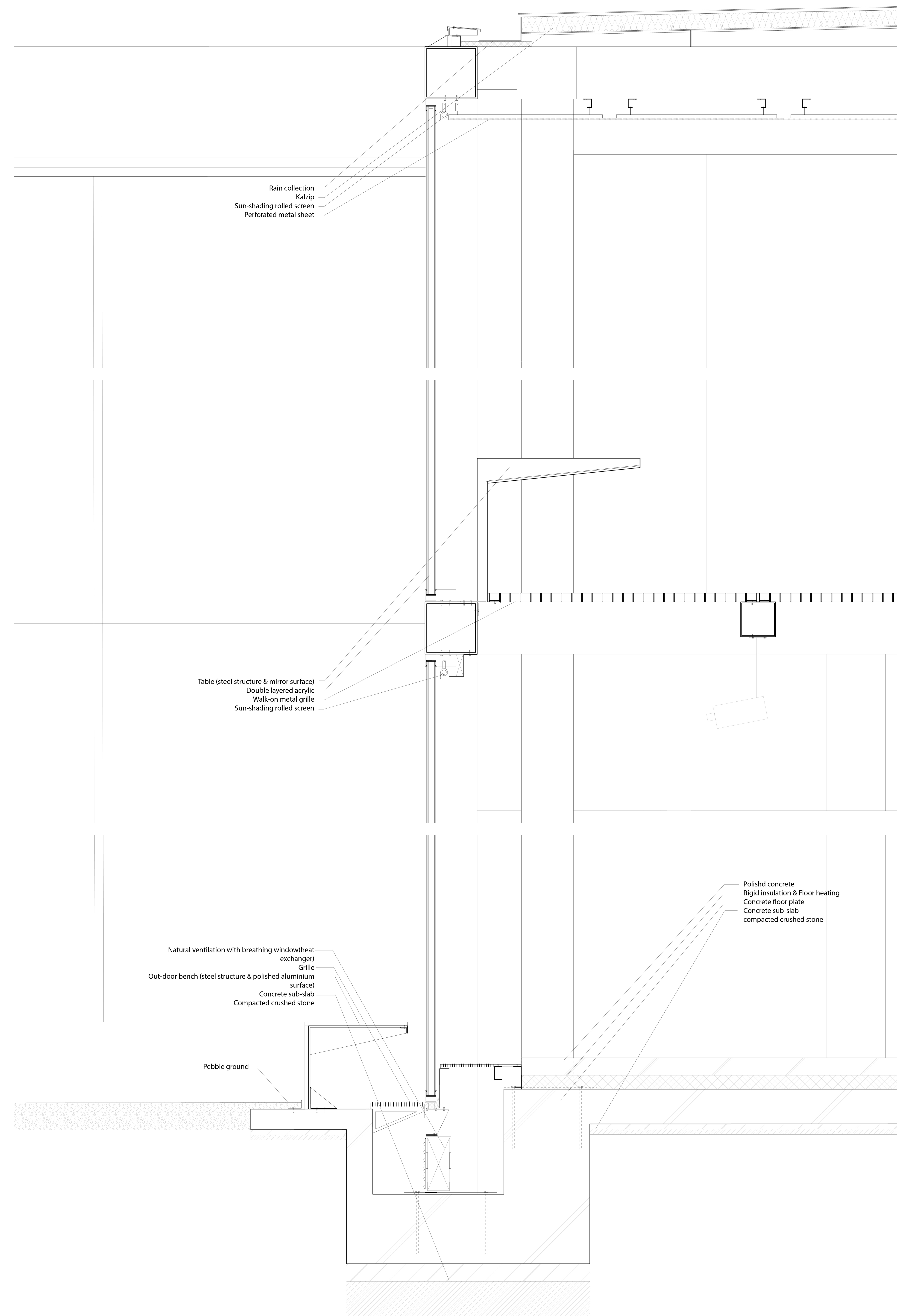
Detail Section_ Ghost Street 1:10
