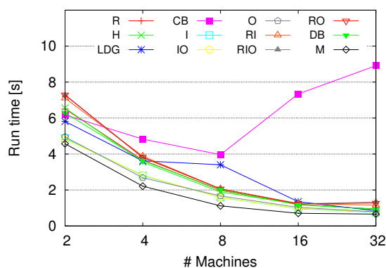
Figure 5.11: The scalability of the WCC algorithm for Datagen_p10m.
