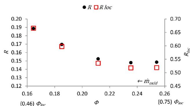
Figure 11. Recirculation ratio and local recirculation ratio as functions of the global equivalence ratio.
