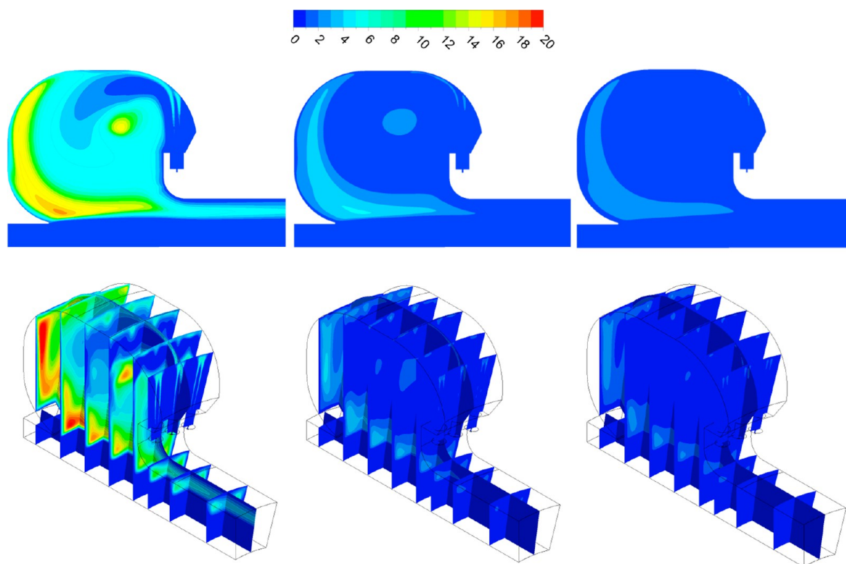
Figure 12. Calculated Da for the without nitrogen addition (left), with 80 l_n/\text{min} N_2 addition (middle) and 100 l_n/\text{min} (right). Lateral (up) and isometric (down) views. Nonadiabatic CFD simulations.
