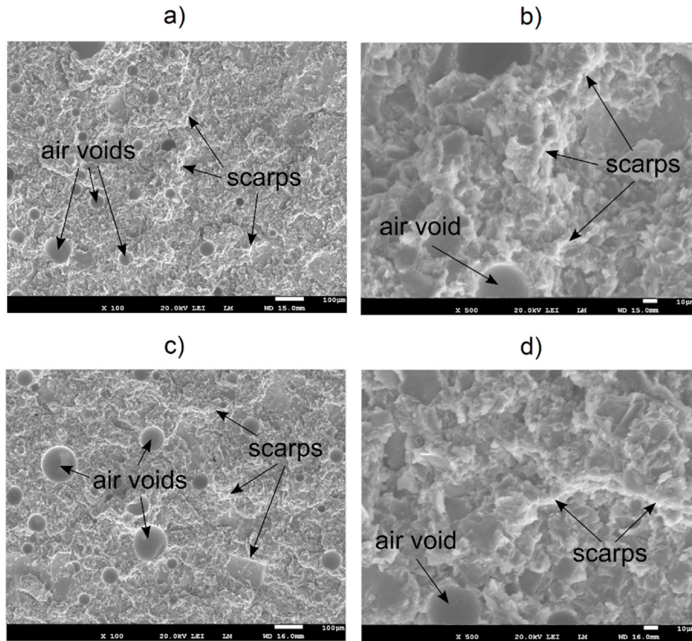
Fig. 14. SEM images of non-aged specimen tested with c = 110 mm (20% mode II) at (a) x100 and (b) x500 and tested with c = 150 (15% mode II) mm at (c) x100 and (d) x500.
