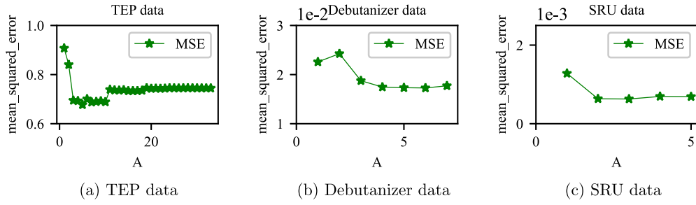
Fig. 5. The influence of latent variable space dimension on prediction results.
