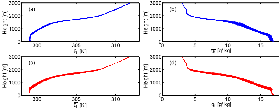
Figure 2.7: Superimposed vertical profiles of \bar{\theta}_l and \bar{q}_t of (a, b) 256 LES subdomains and (c, d) 256 independent SCM-CMC realizations after four hours of integration in the second experiment
