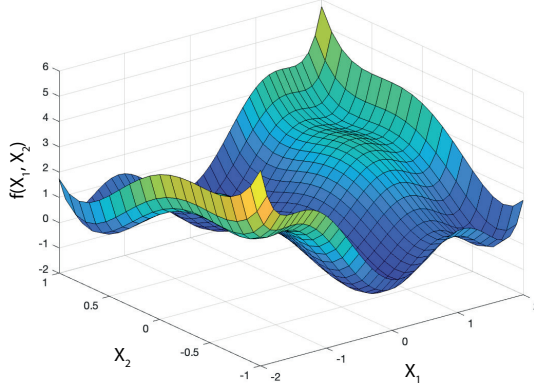
Figure 5.3: Visualization of the six-hump camel function.
