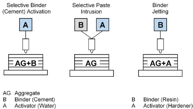
Figure 12. Schematics of powder, reprinted from (Lowke et al., 2018)
