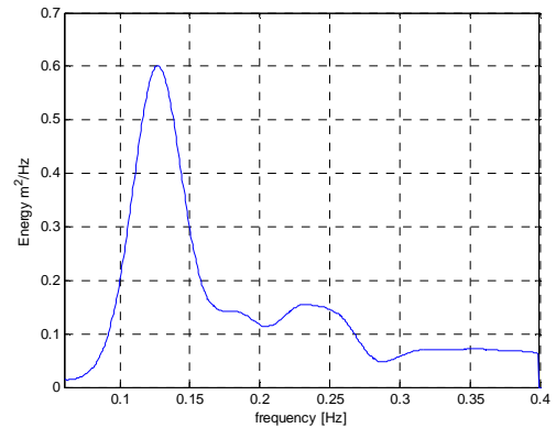
Figure A.15 Wave spectrum of Bardex07
