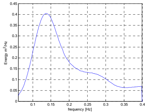
Figure A.9 Wave spectrum of Bardex04
