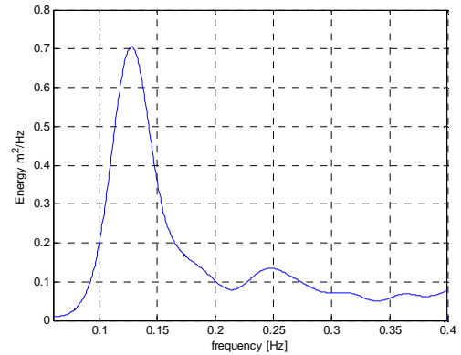
Figure A.13 Wave spectrum of Bardex06
