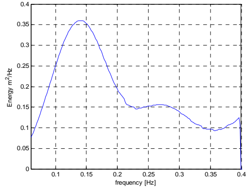
Figure A.3 Wave spectrum of Bardex01
