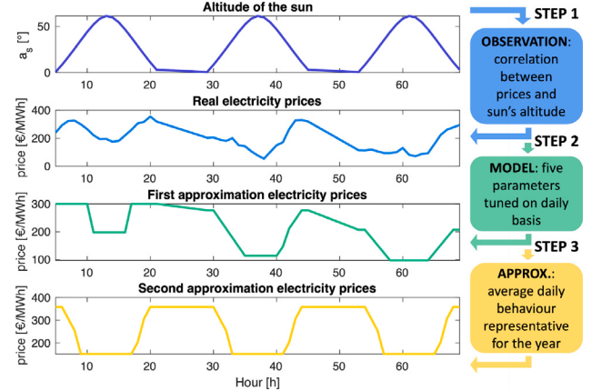
Fig. 5. Main steps in the modelling of the electricity prices. This example refers to the period 16–18 June 2022 of the Netherlands.
